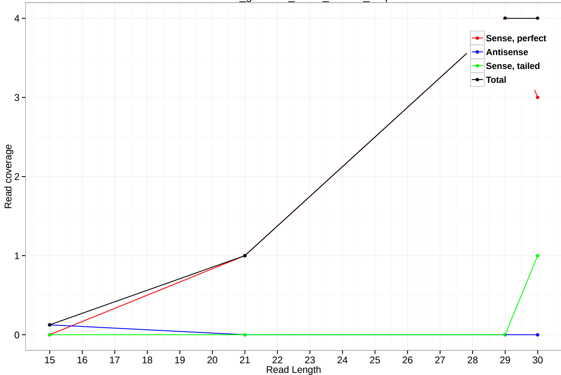
rheMac3_genscan_chr14_126.23_9.3p
