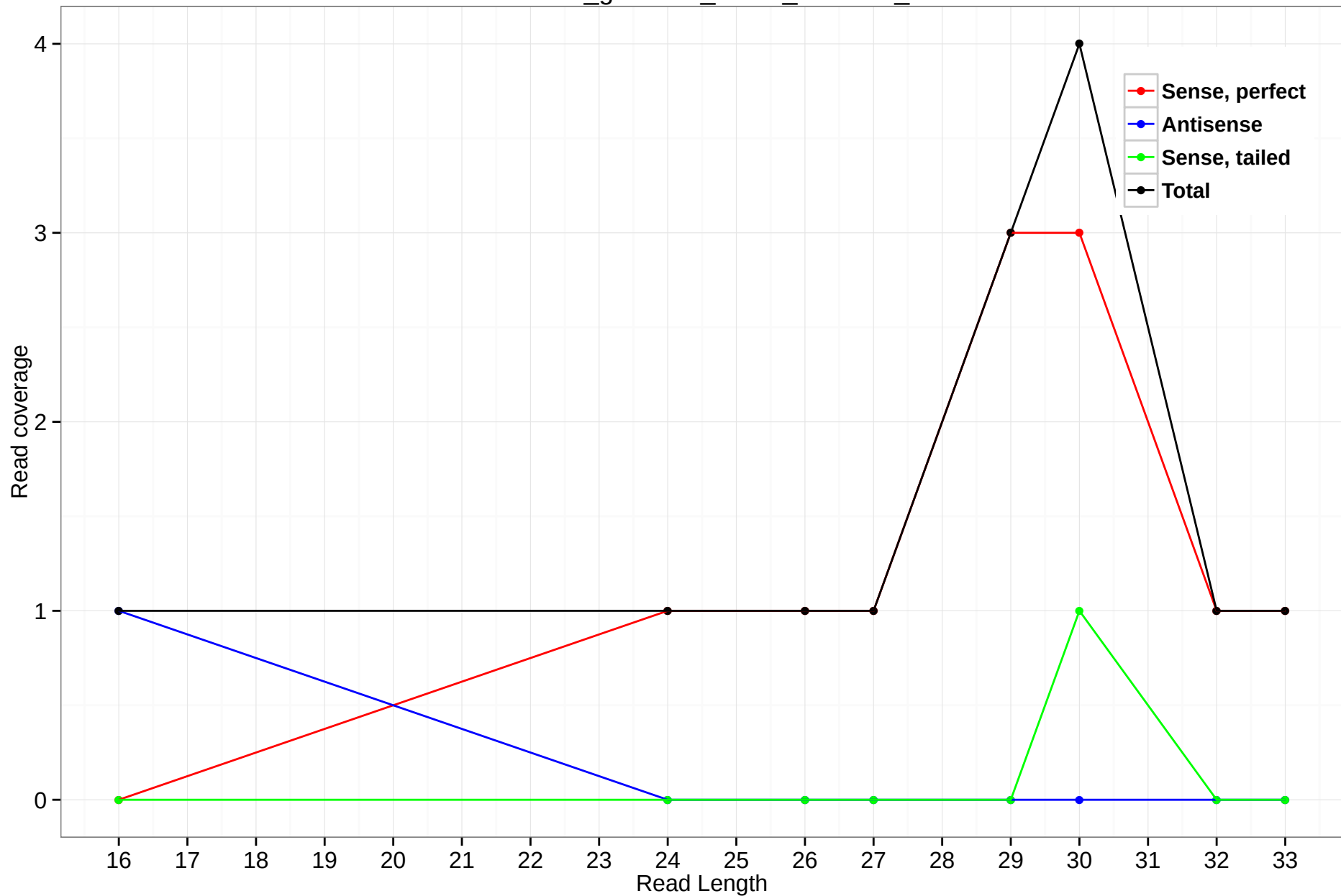
rheMac3_genscan_chr14_126.107_3
