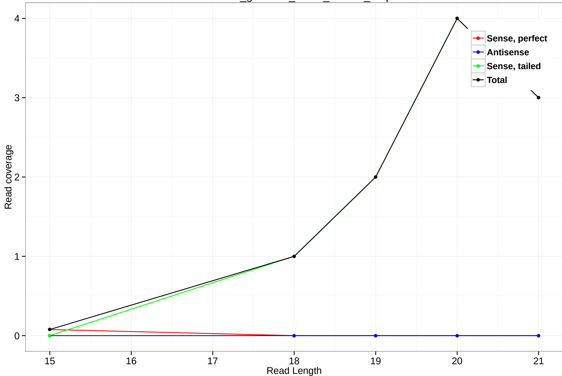
rheMac3_genscan_chr14_124.26_3.3p
