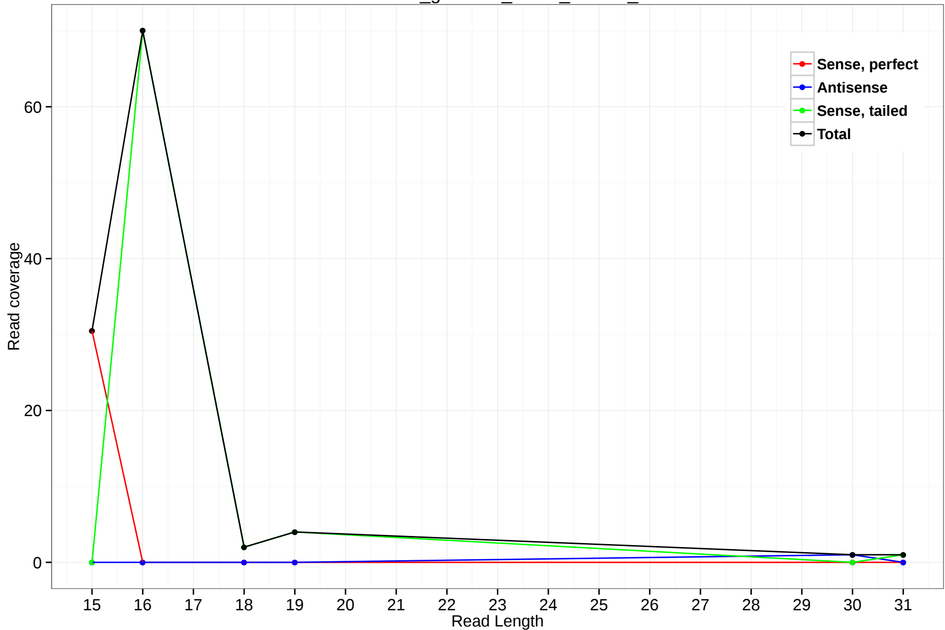
rheMac3_genscan_chr14_124.11_4
