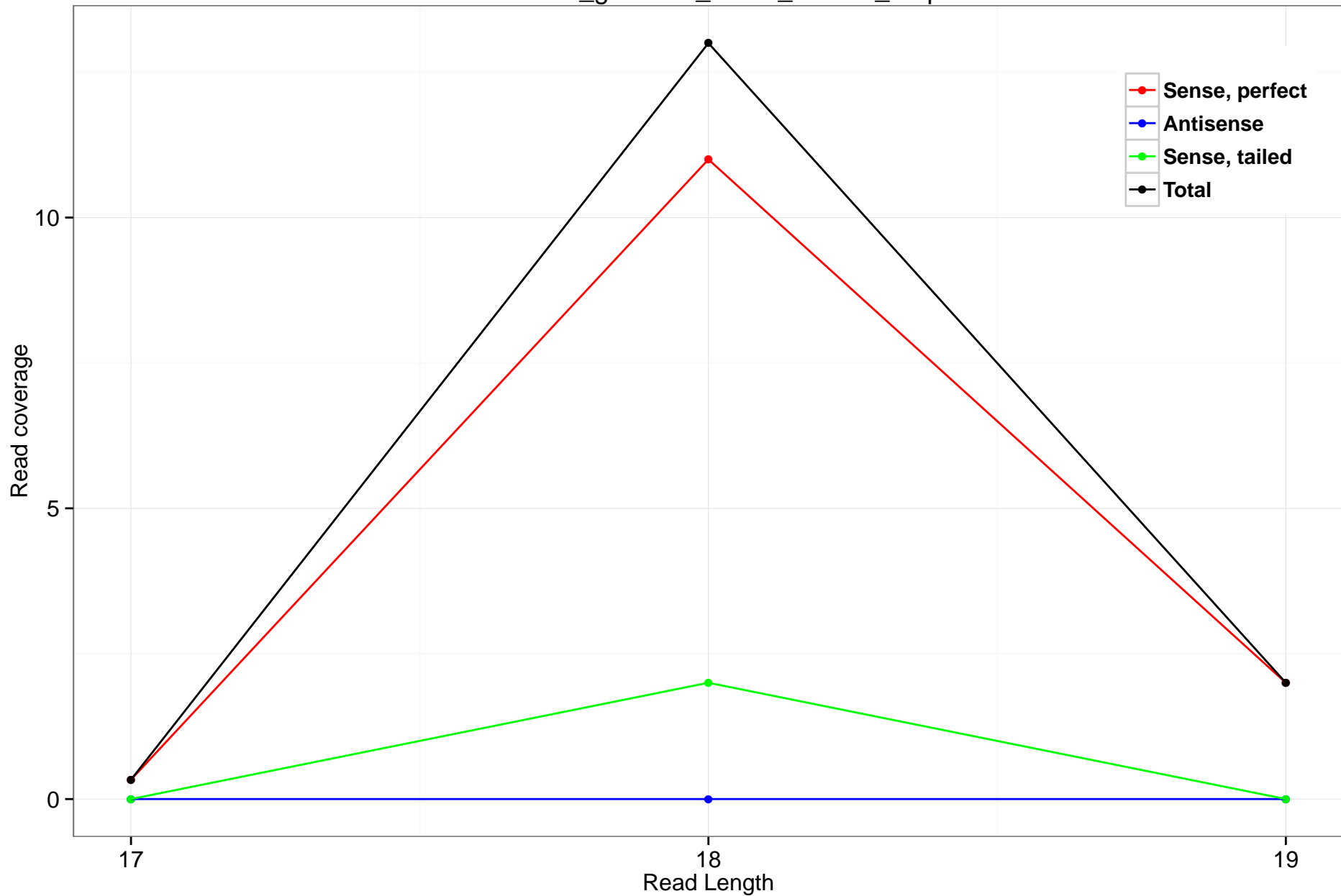
rheMac3_genscan_chr14_122.41_2.3p
