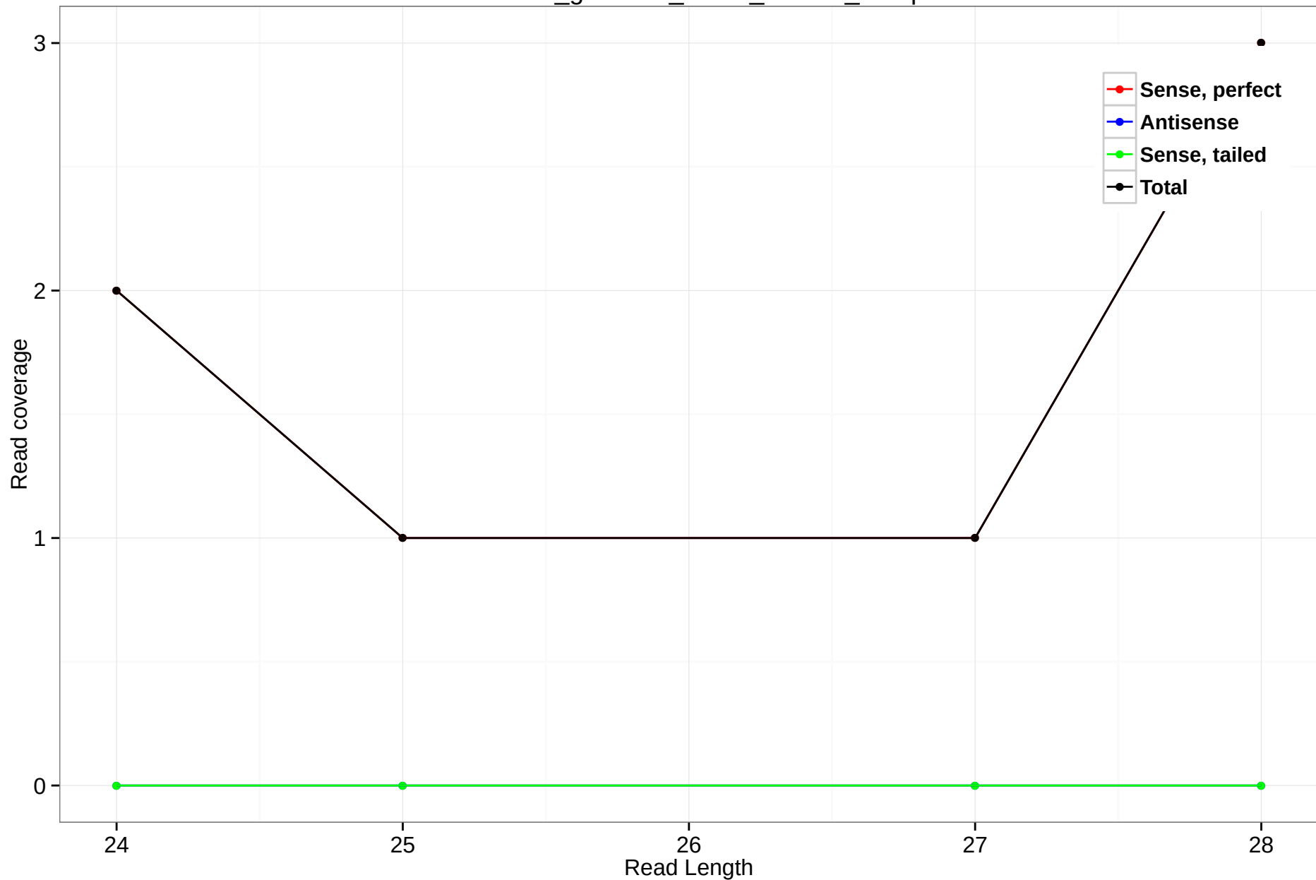
rheMac3_genscan_chr14_119.89_33.5p
