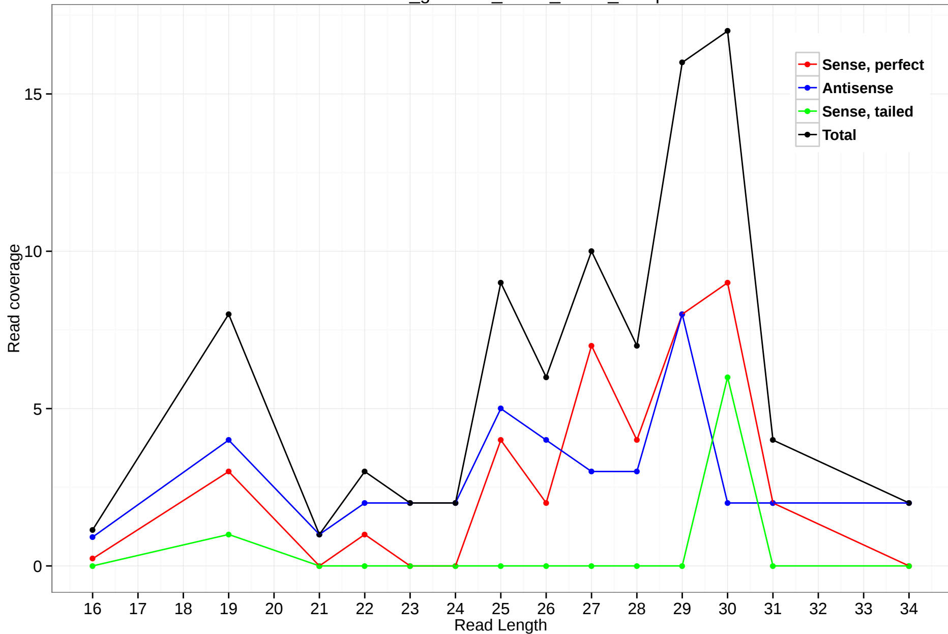
rheMac3_genscan_chr14_119.7_12.3p
