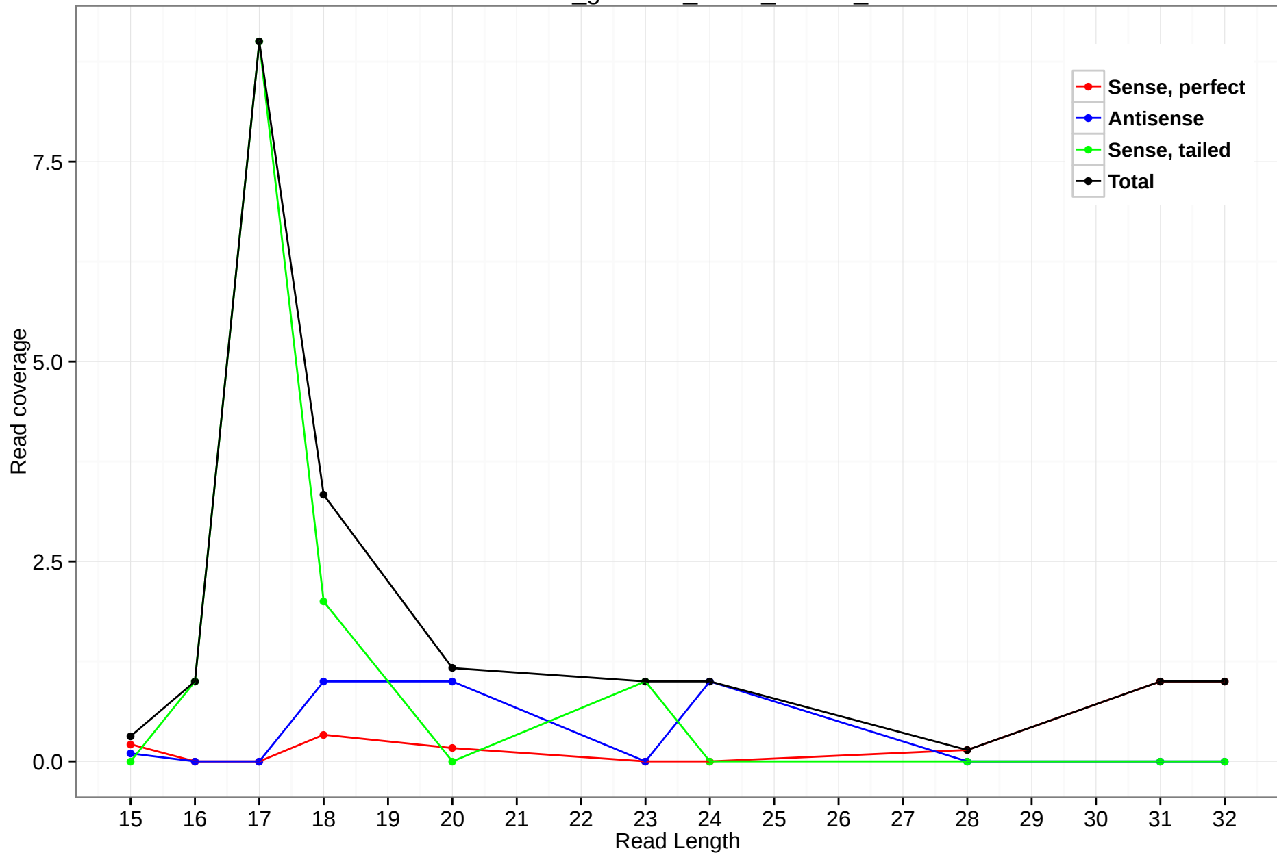
rheMac3_genscan_chr14_119.66_1
