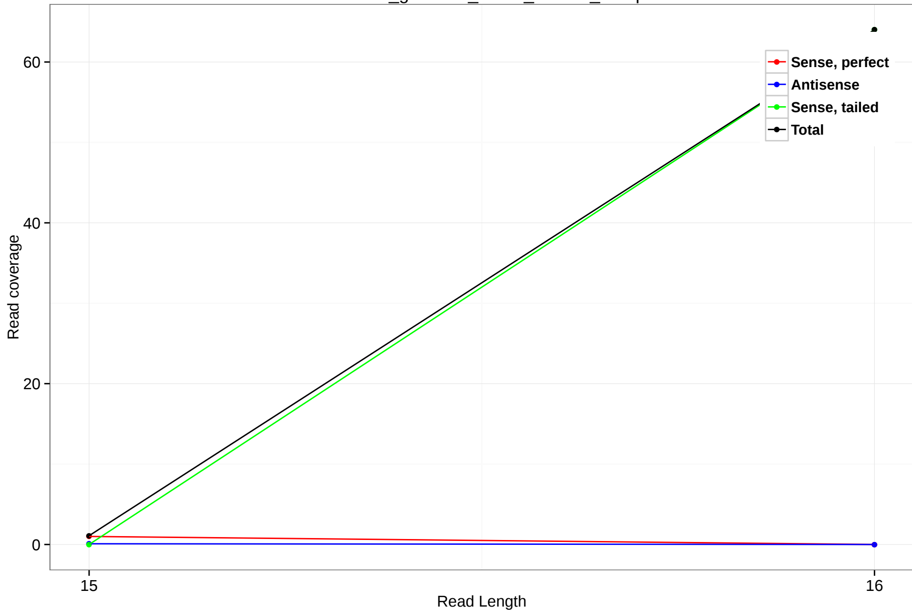
rheMac3_genscan_chr14_119.11_17.3p
