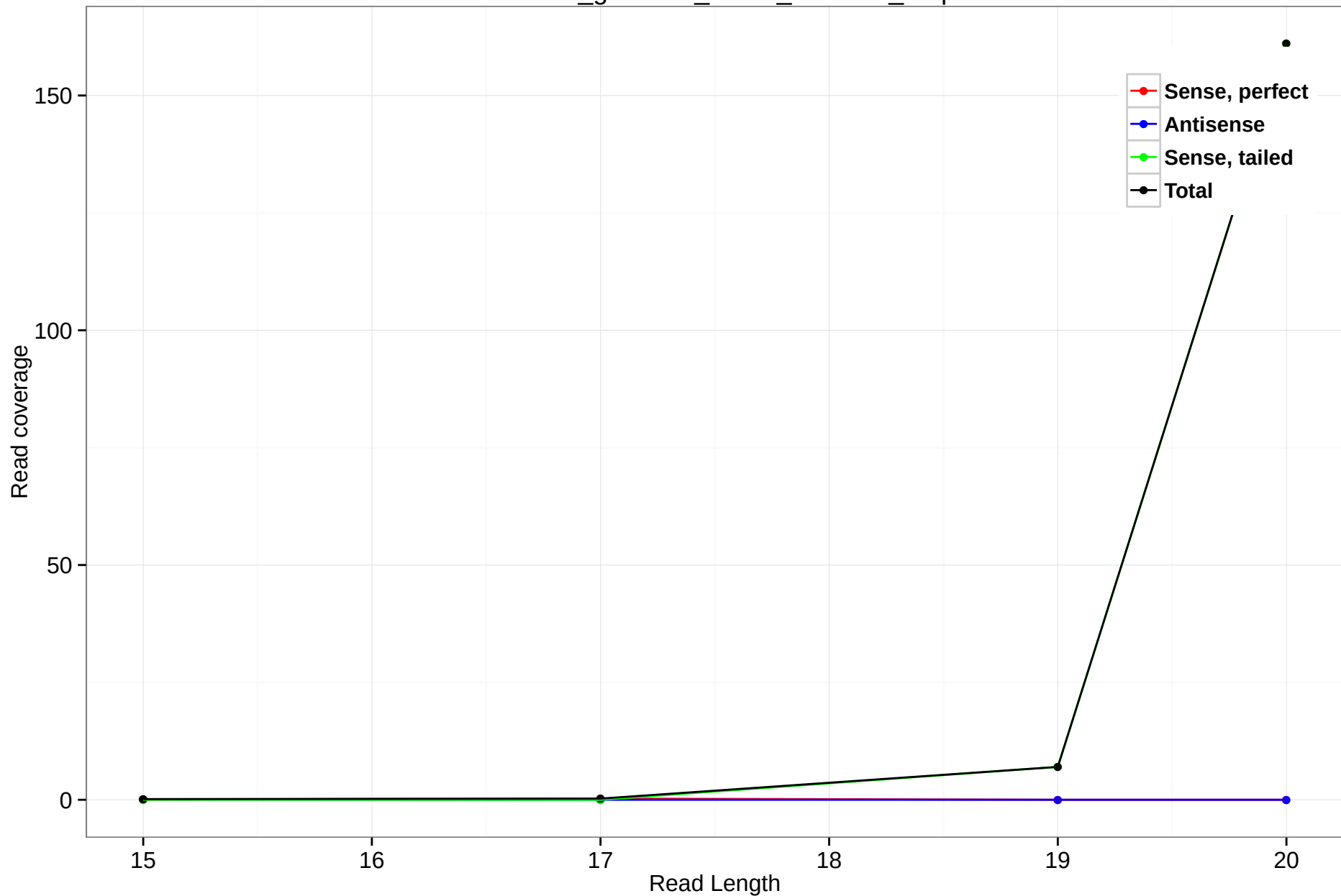
rheMac3_genscan_chr14_119.114_3.5p
