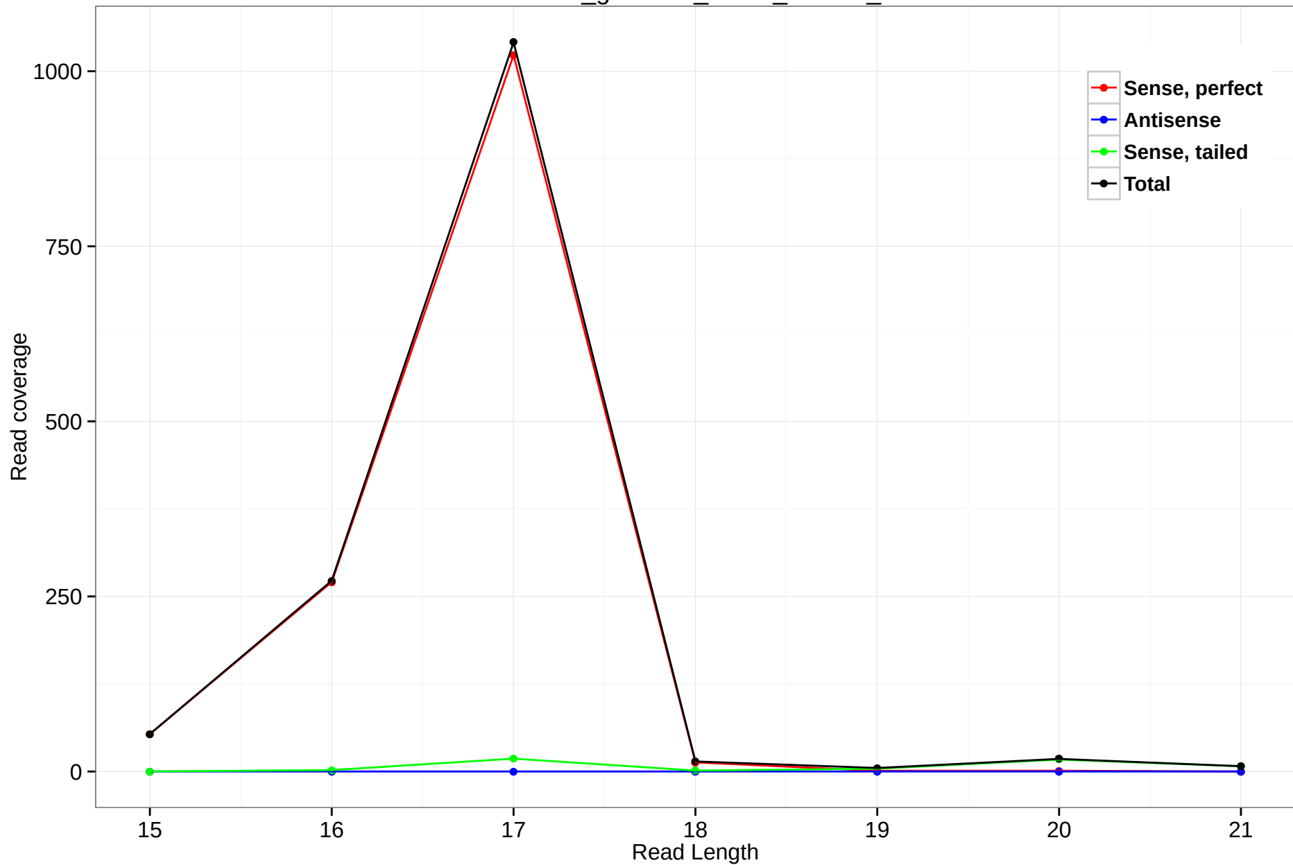
rheMac3_genscan_chr14_118.92_16
