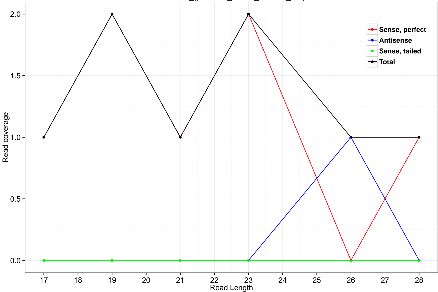
rheMac3_genscan_chr14_118.90_0.3p
