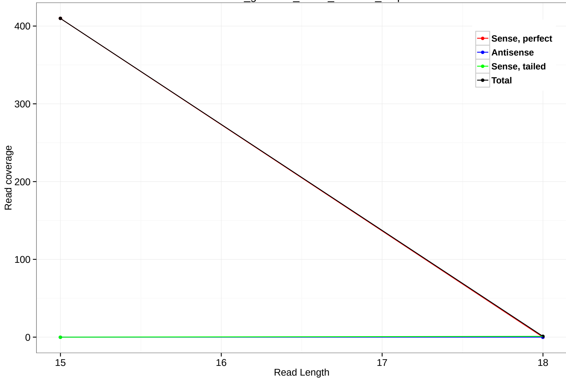
rheMac3_genscan_chr14_118.108_9.5p
