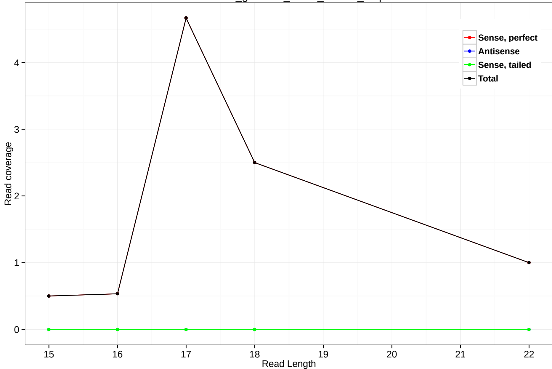
rheMac3_genscan_chr14_116.15_0.3p
