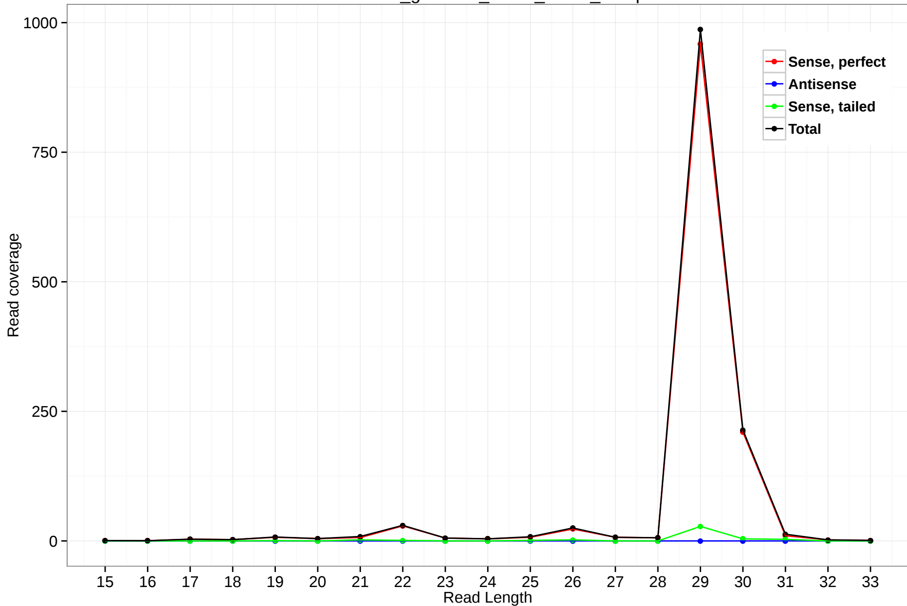
rheMac3_genscan_chr14_106.6_14.5p
