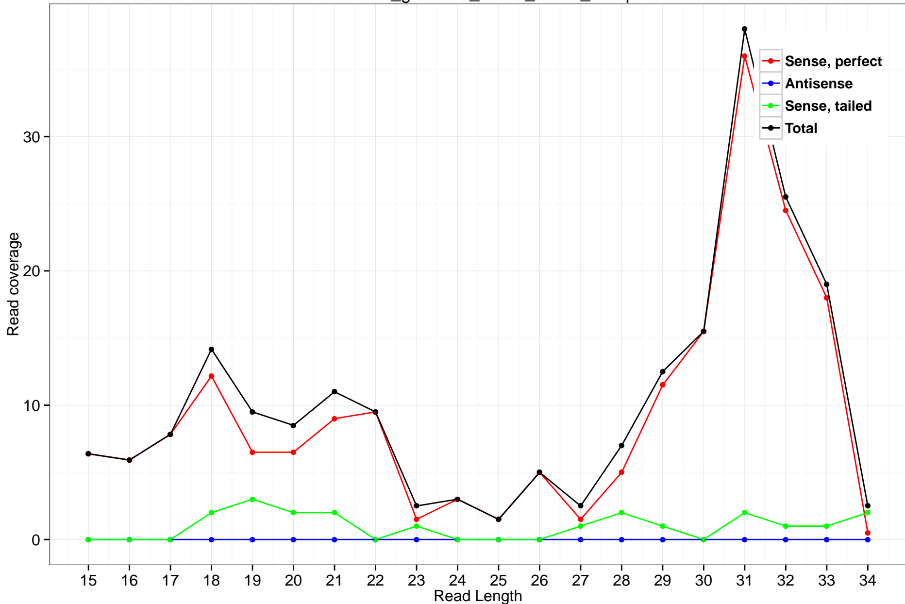
rheMac3_genscan_chr14_106.6_14.3p
