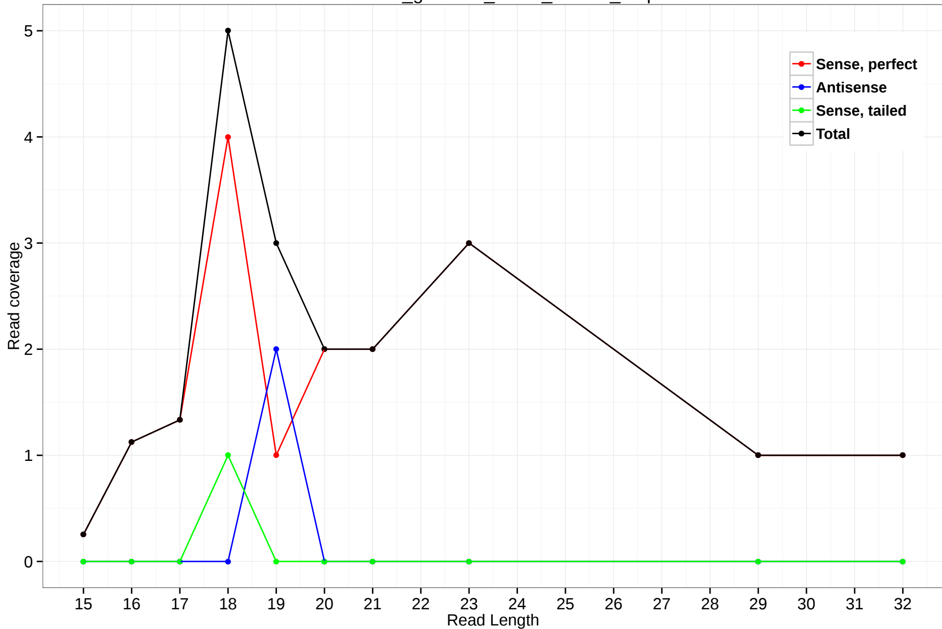
rheMac3_genscan_chr14_106.34_1.5p
