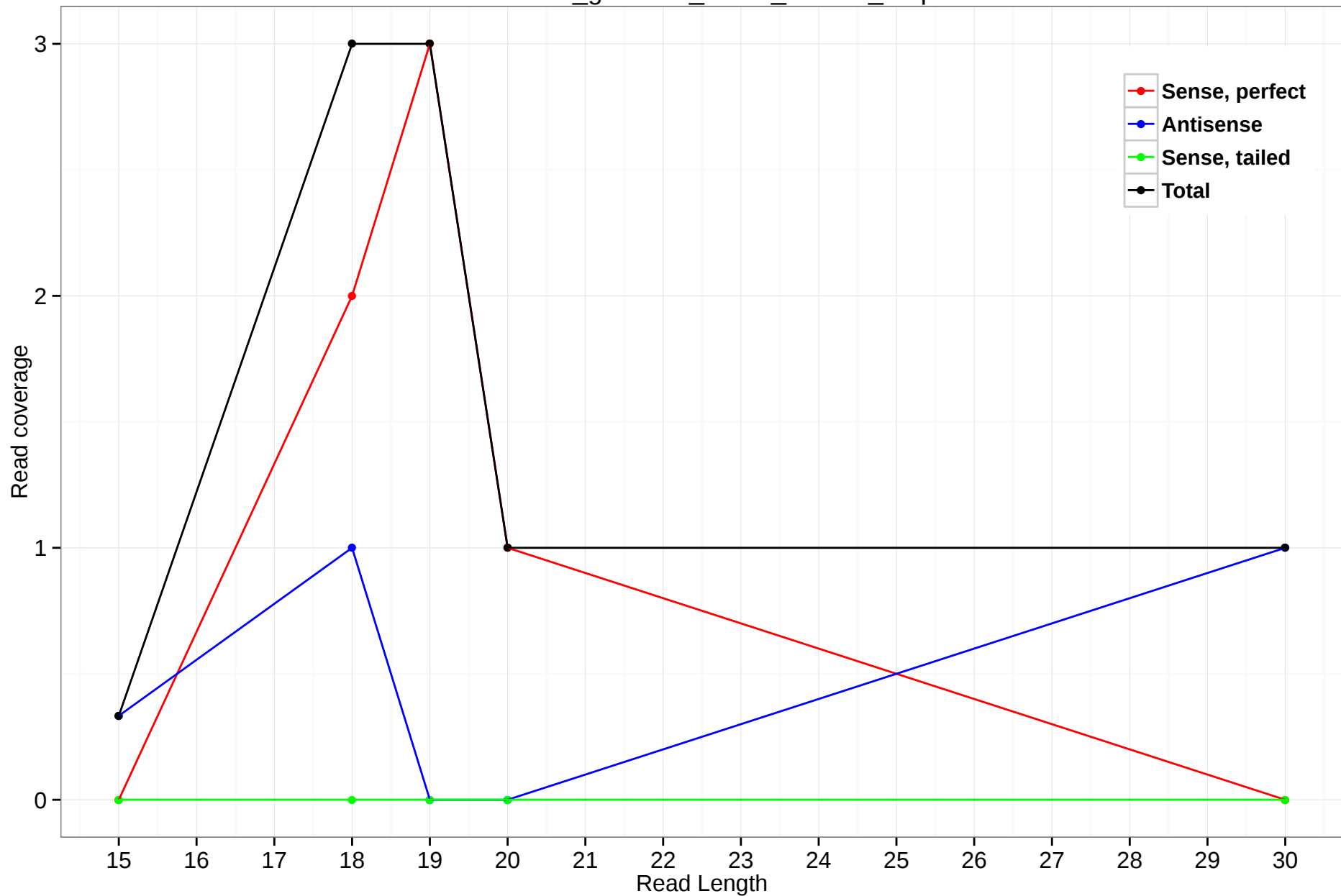
rheMac3_genscan_chr14_106.17_4.5p
