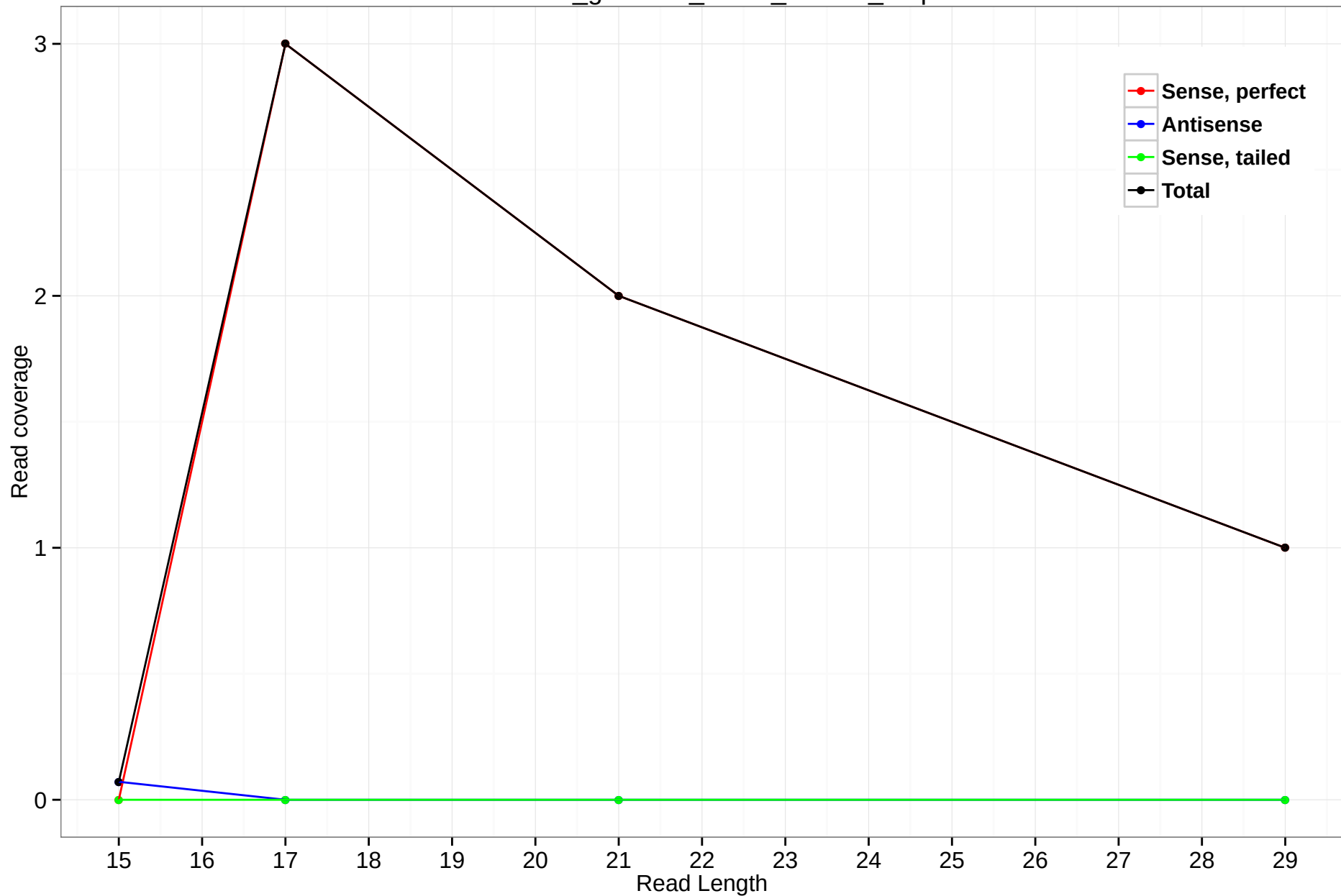
rheMac3_genscan_chr14_104.38_3.5p
