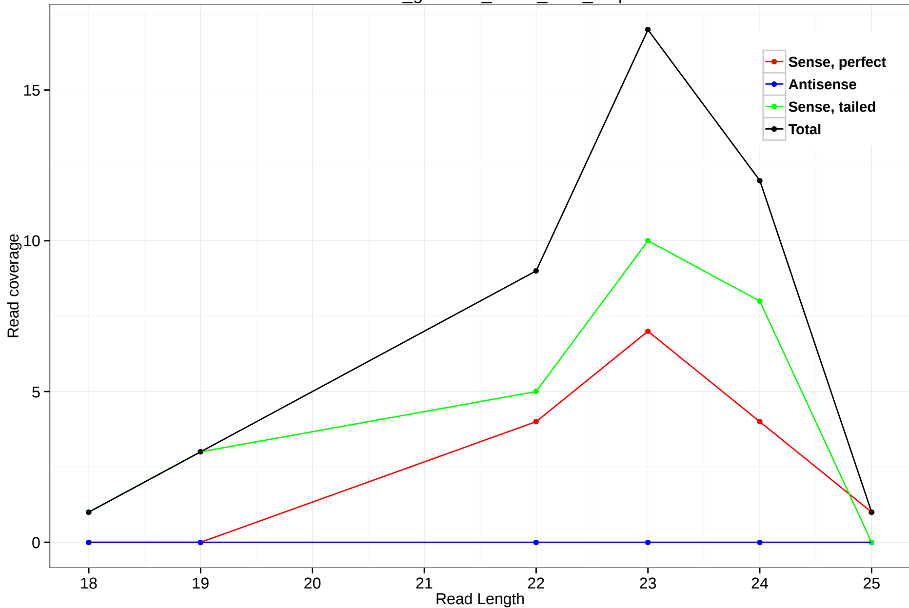
rheMac3_genscan_chr14_06.9_2.3p
