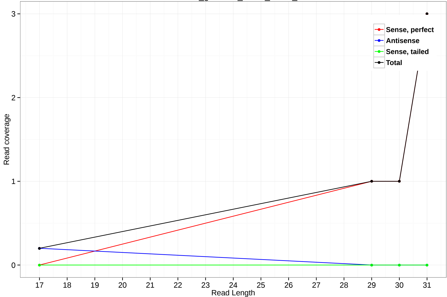
rheMac3_genscan_chr14_06.54_6
