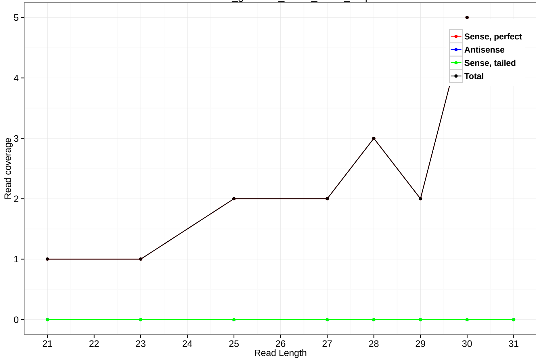
rheMac3_genscan_chr14_06.36_9.3p
