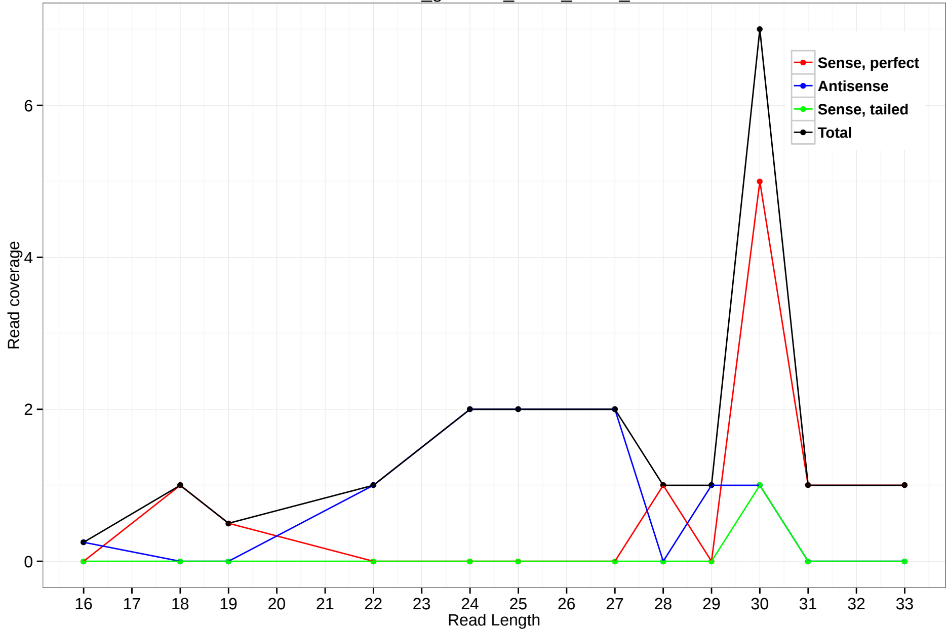
rheMac3_genscan_chr14_06.32_7
