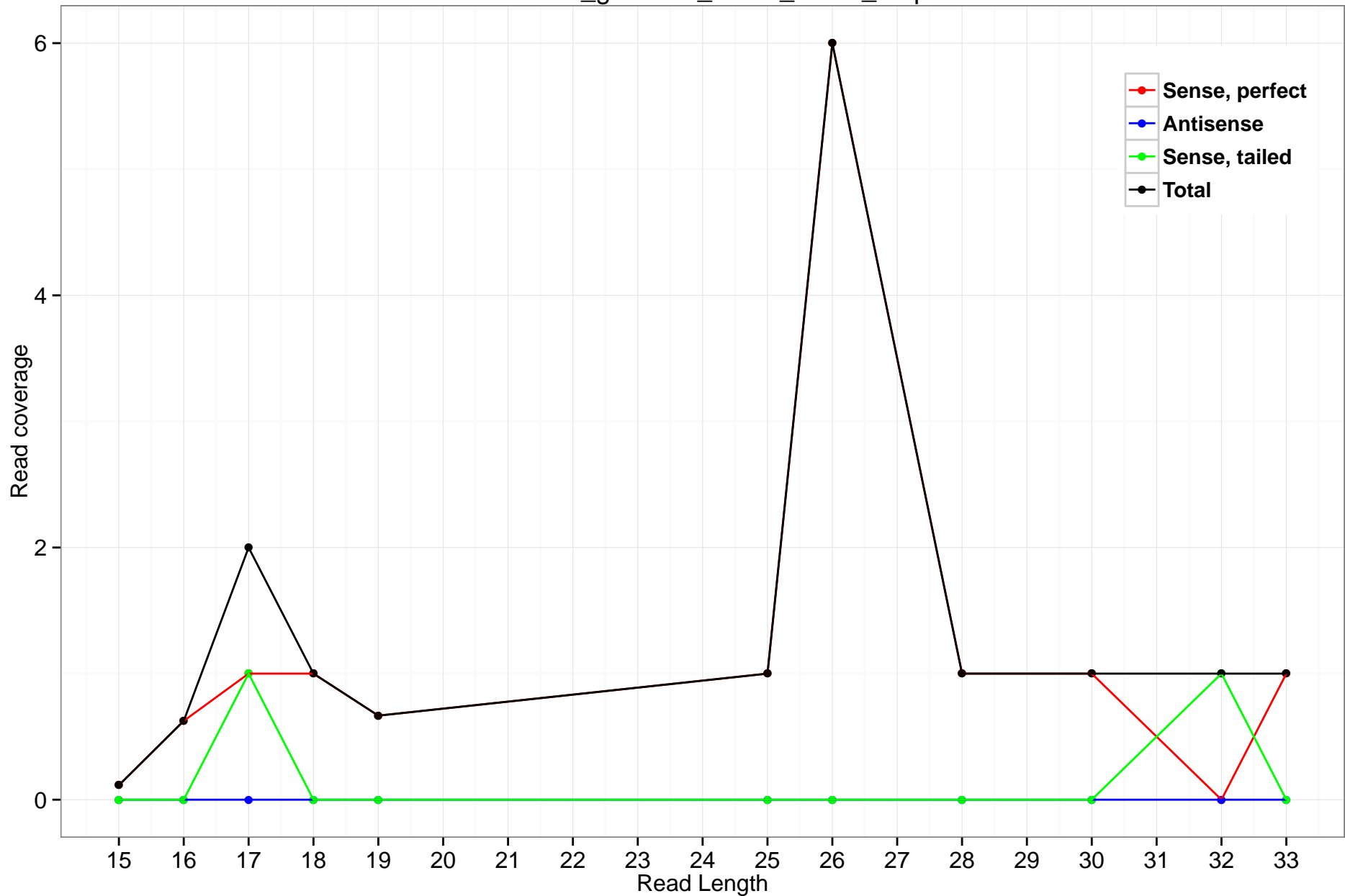
rheMac3_genscan_chr14_06.16_3.3p
