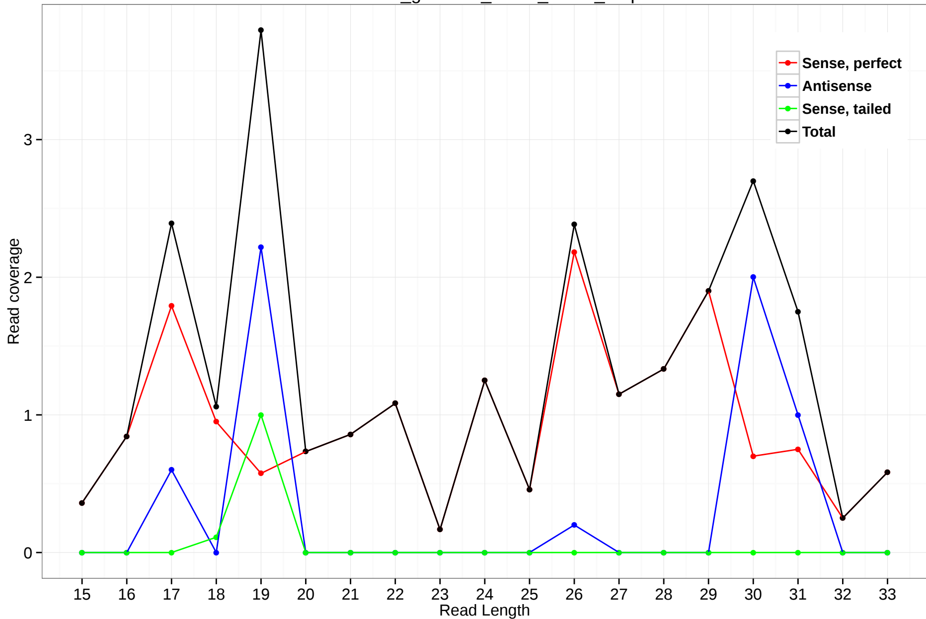
rheMac3_genscan_chr14_06.16_2.3p
