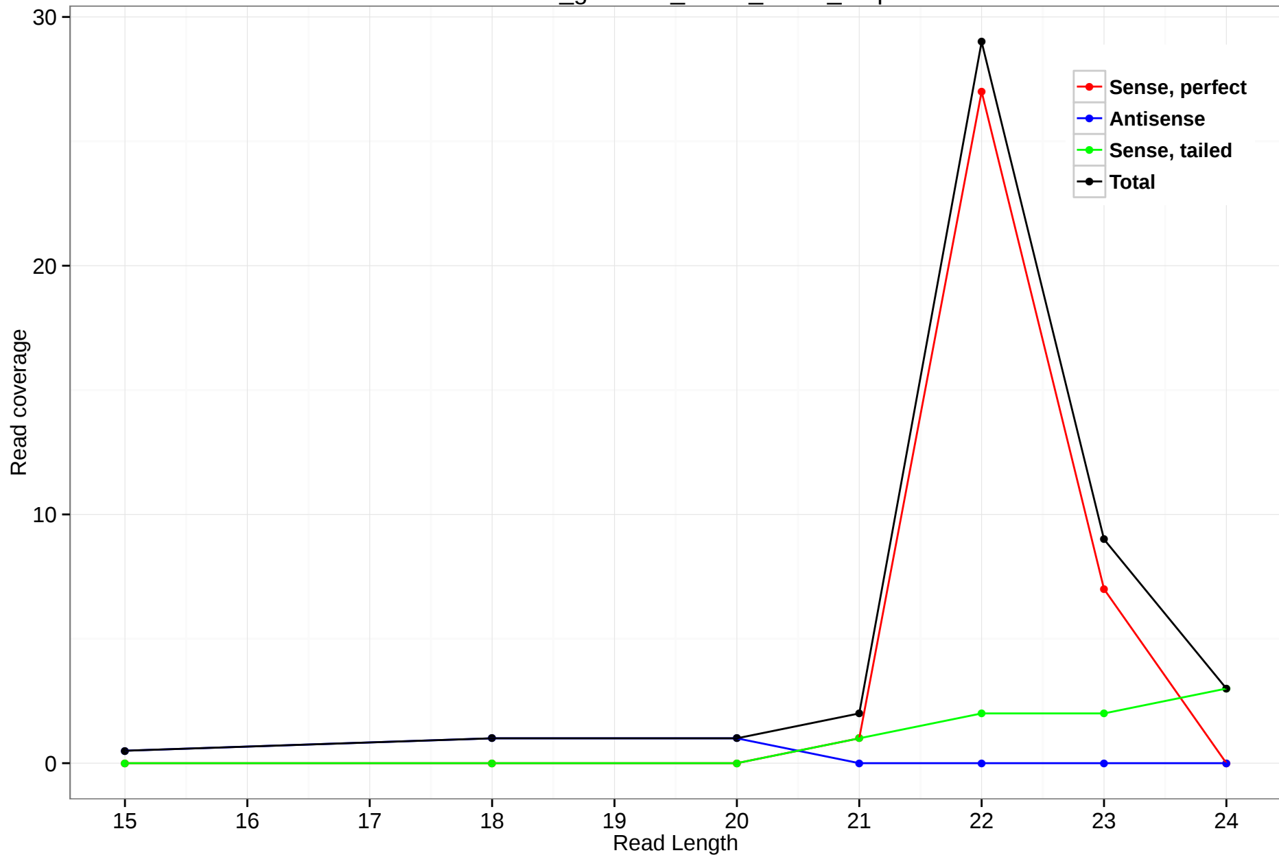
rheMac3_genscan_chr14_05.73_6.5p
