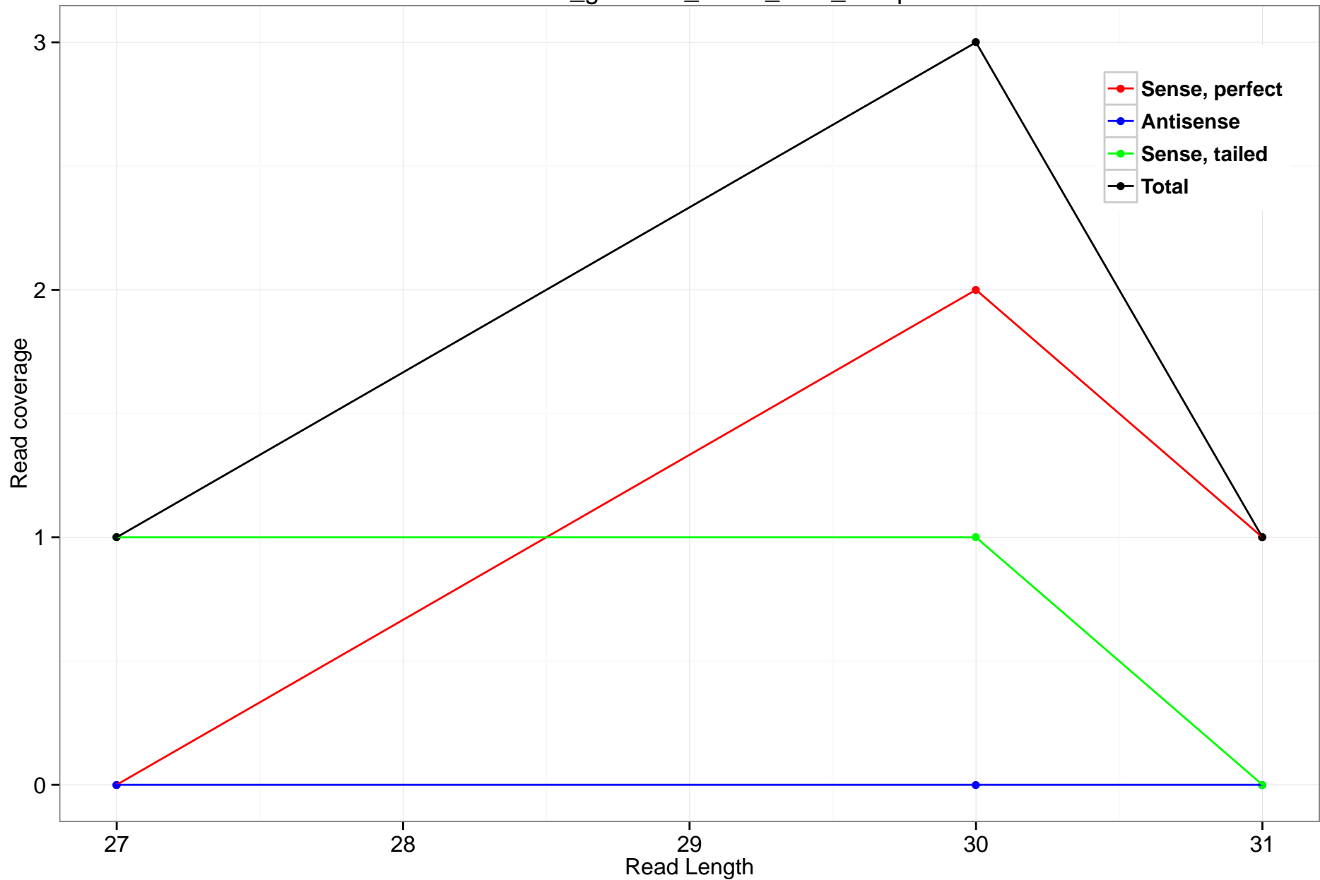
rheMac3_genscan_chr14_05.6_13.3p
