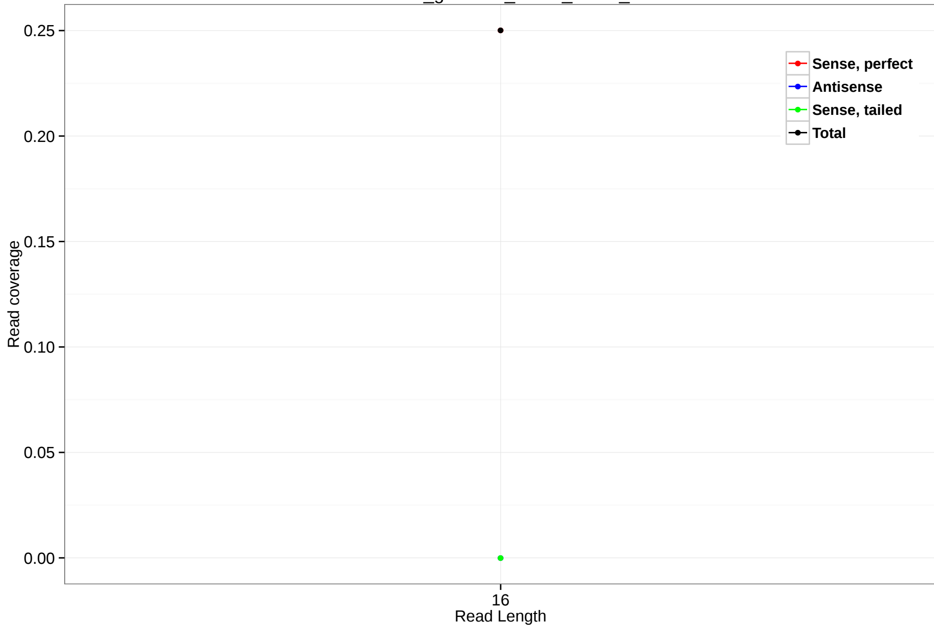
rheMac3_genscan_chr14_05.69_45
