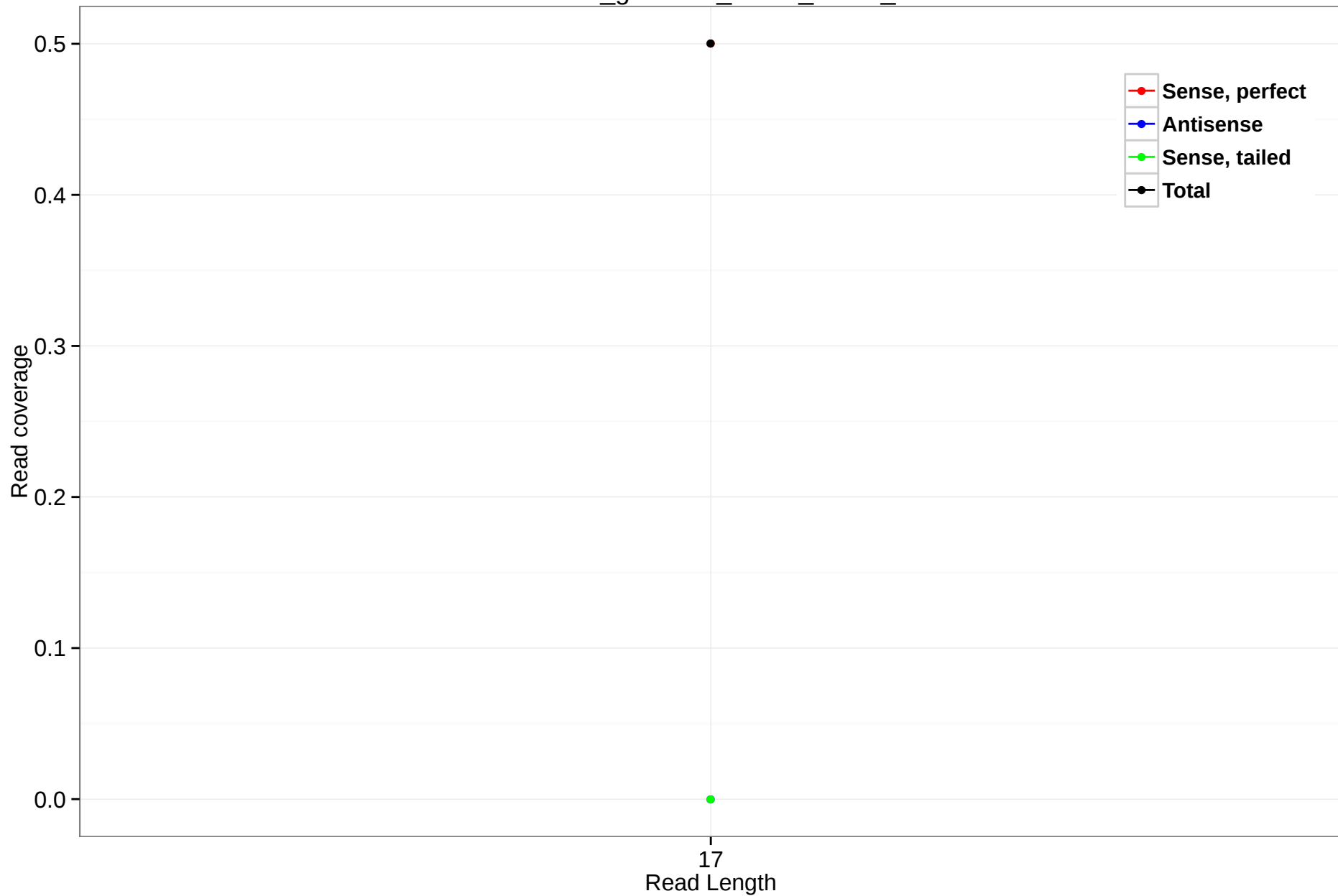
rheMac3_genscan_chr14_05.69_34
