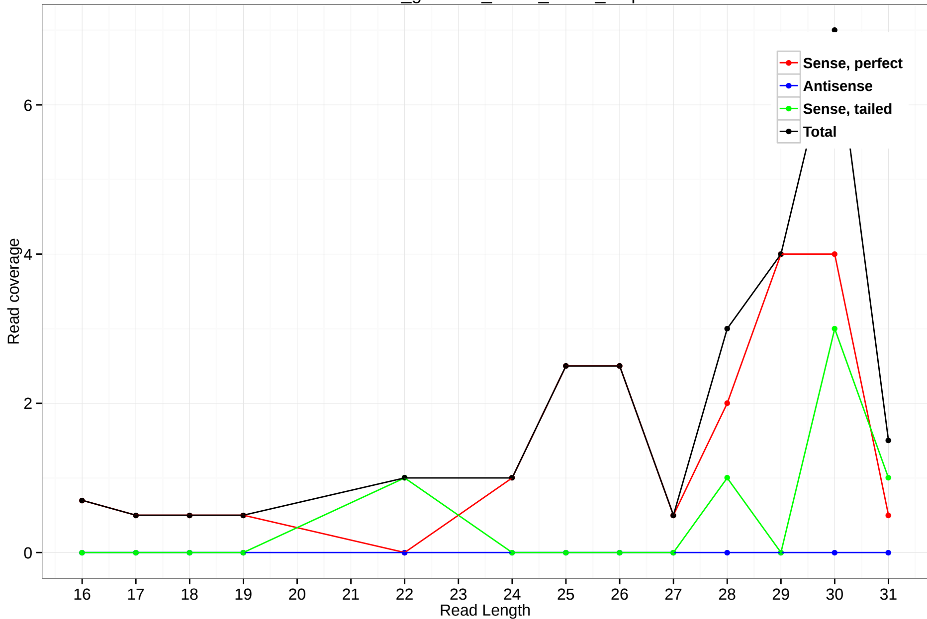
rheMac3_genscan_chr14_05.33_2.5p
