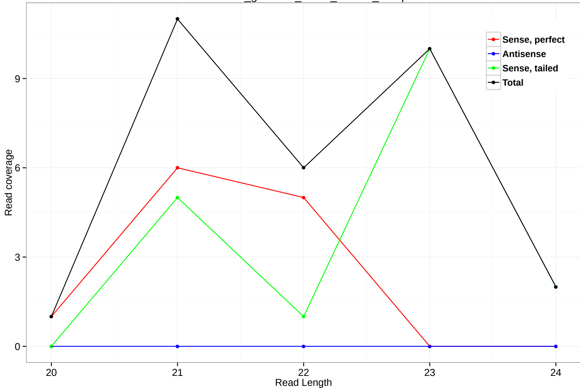
rheMac3_genscan_chr14_05.206_28.3p
