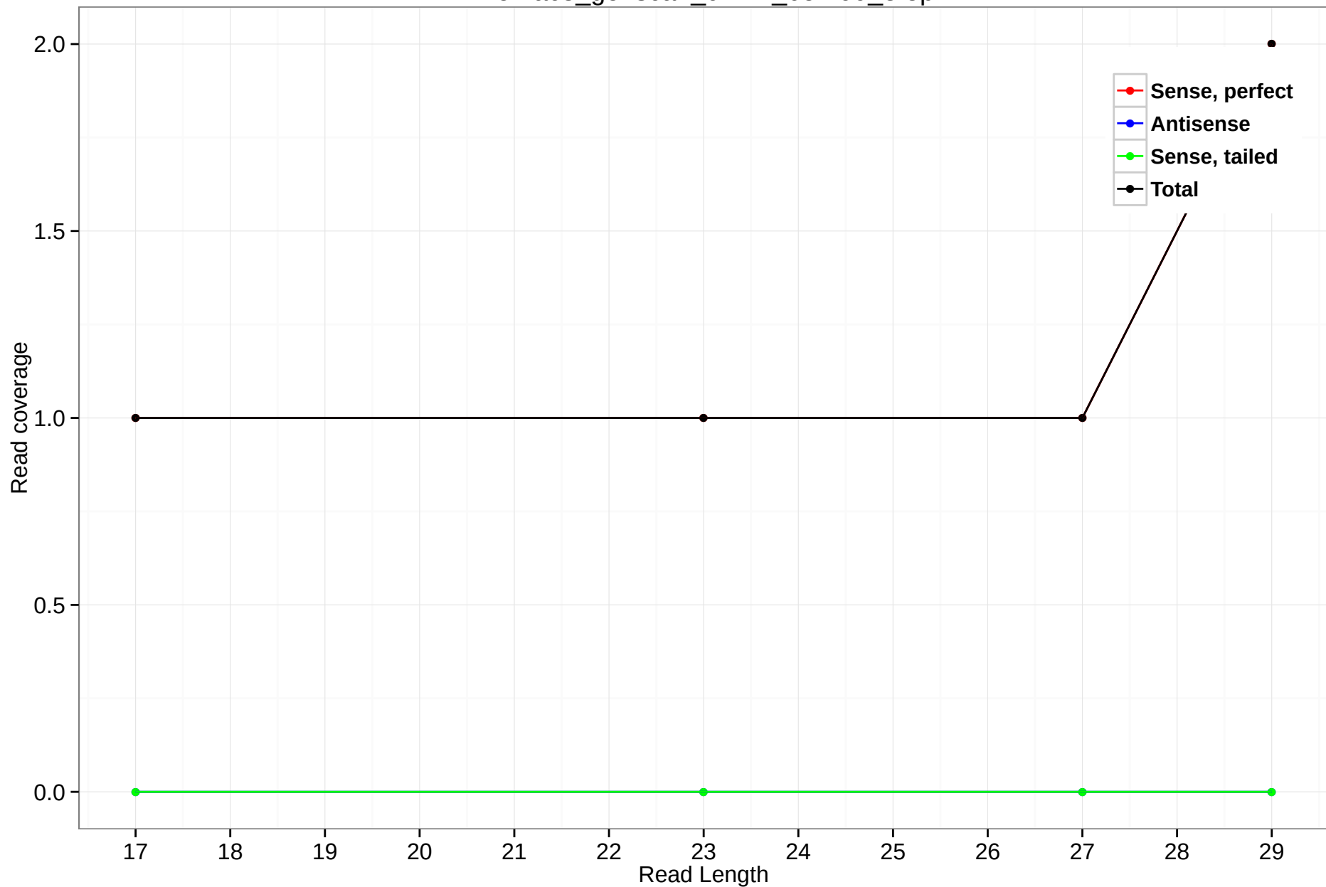
rheMac3_genscan_chr14_05.199_8.5p
