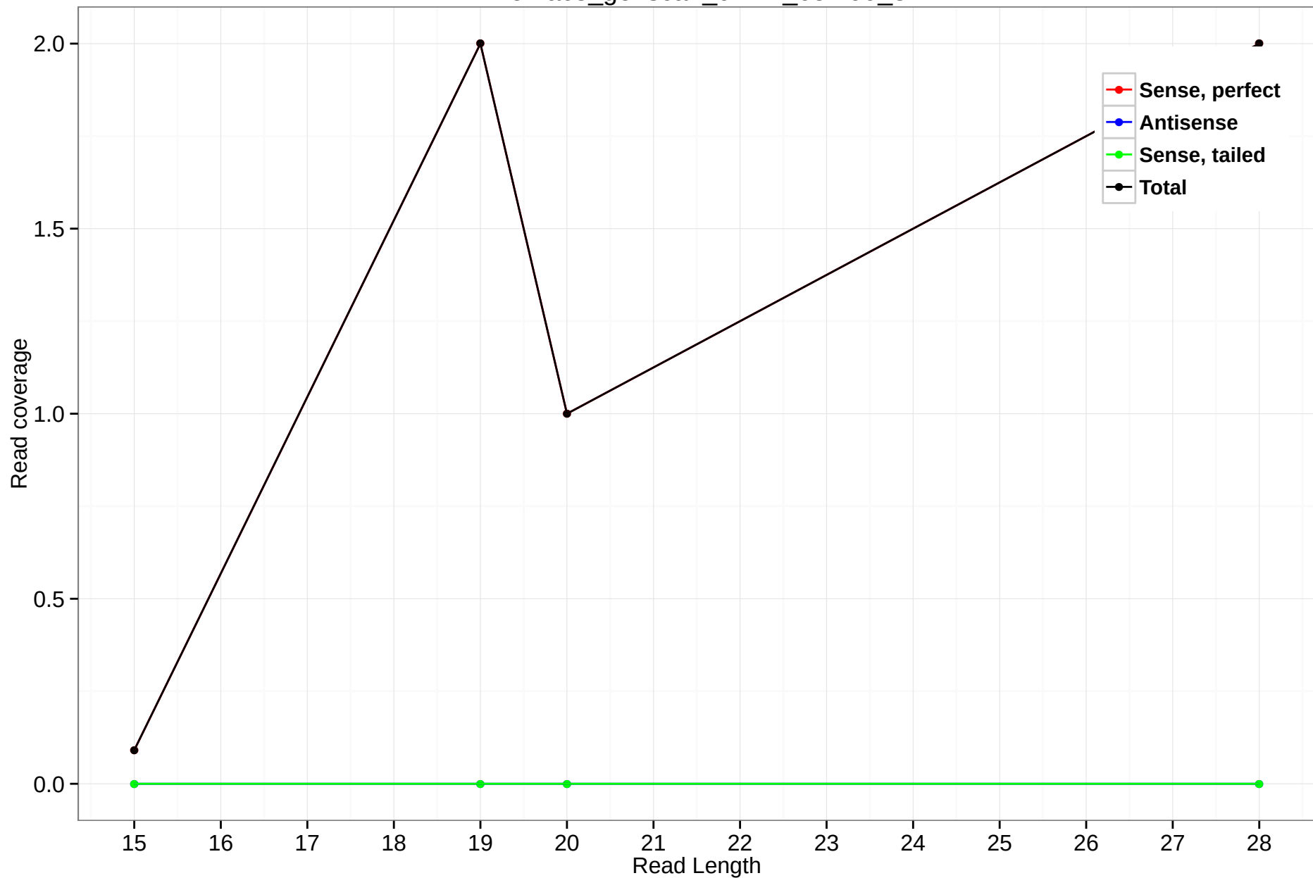
rheMac3_genscan_chr14_05.199_3
