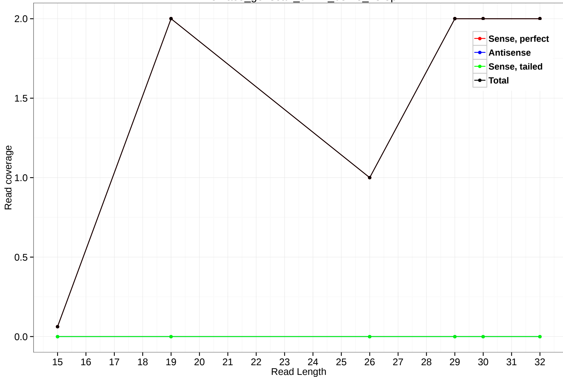
rheMac3_genscan_chr14_05.18_25.5p
