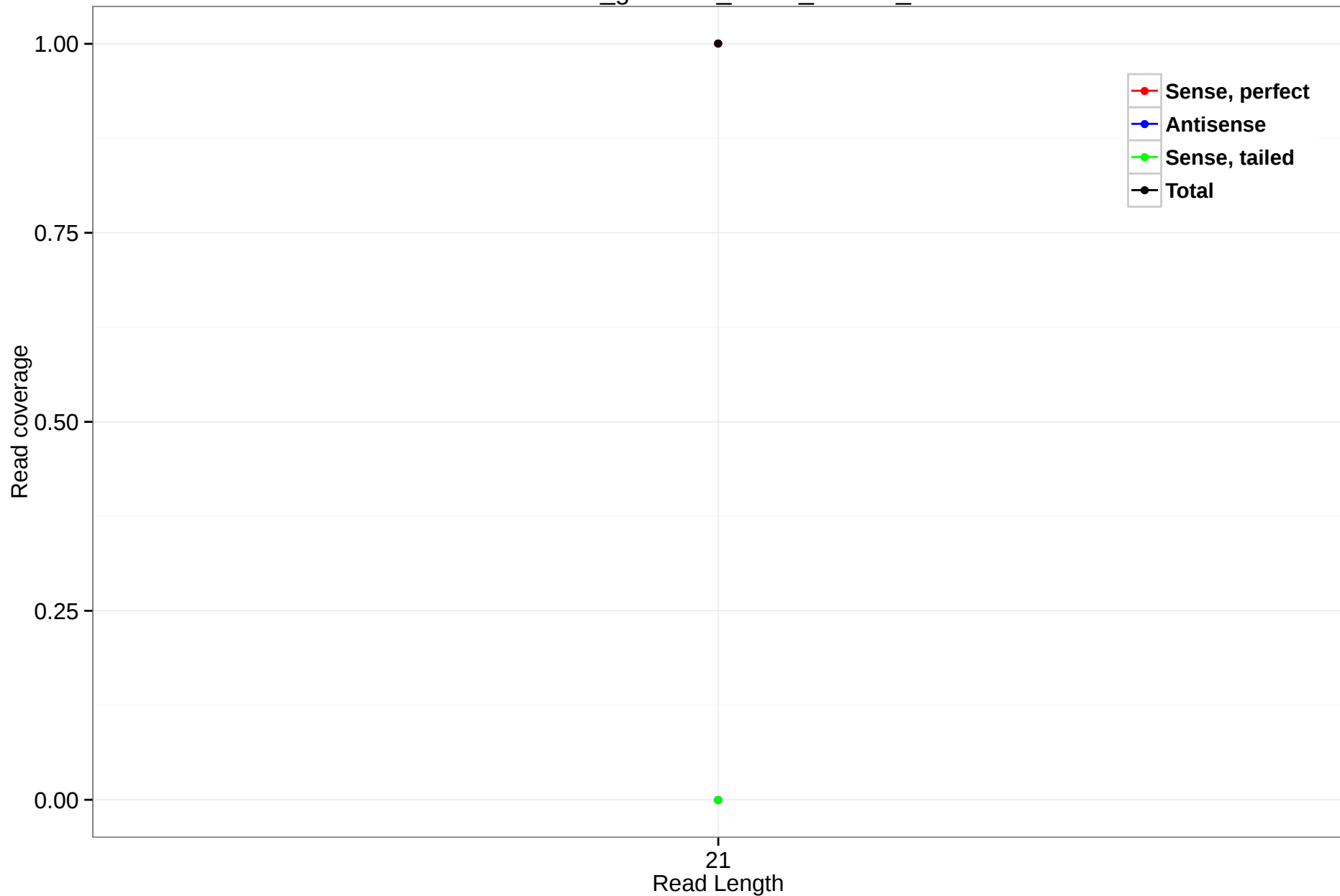
rheMac3_genscan_chr14_05.154_11
