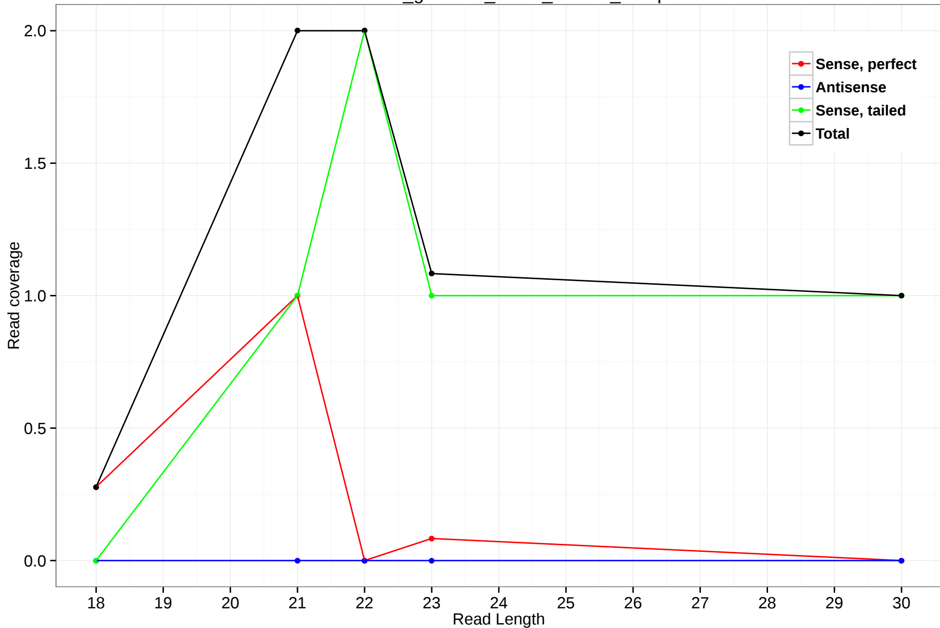
rheMac3_genscan_chr14_05.153_16.3p
