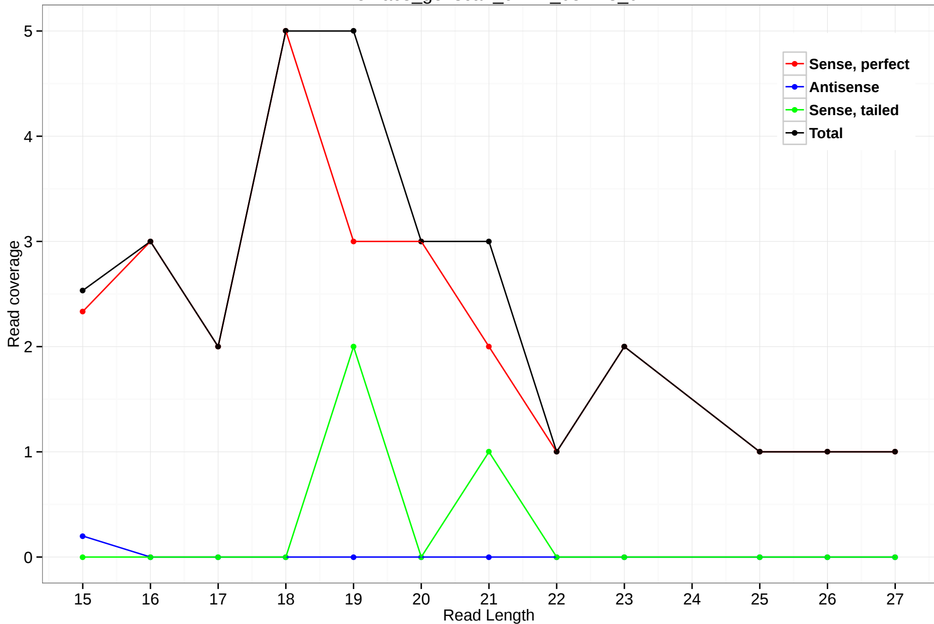
rheMac3_genscan_chr14_05.143_0
