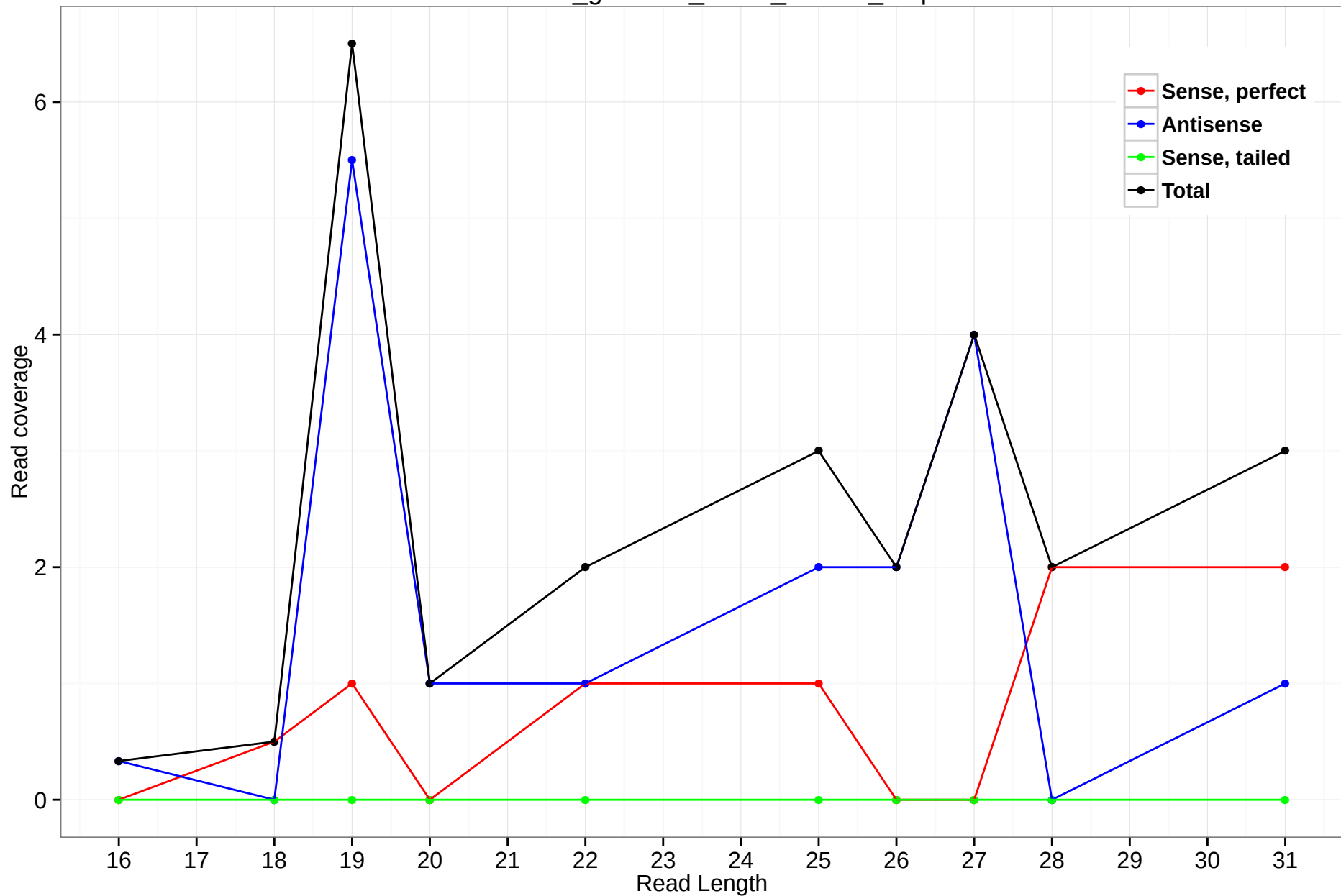
rheMac3_genscan_chr14_05.135_4.3p
