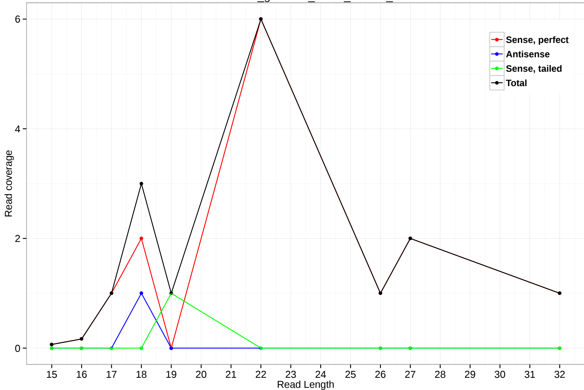
rheMac3_genscan_chr14_05.130_7
