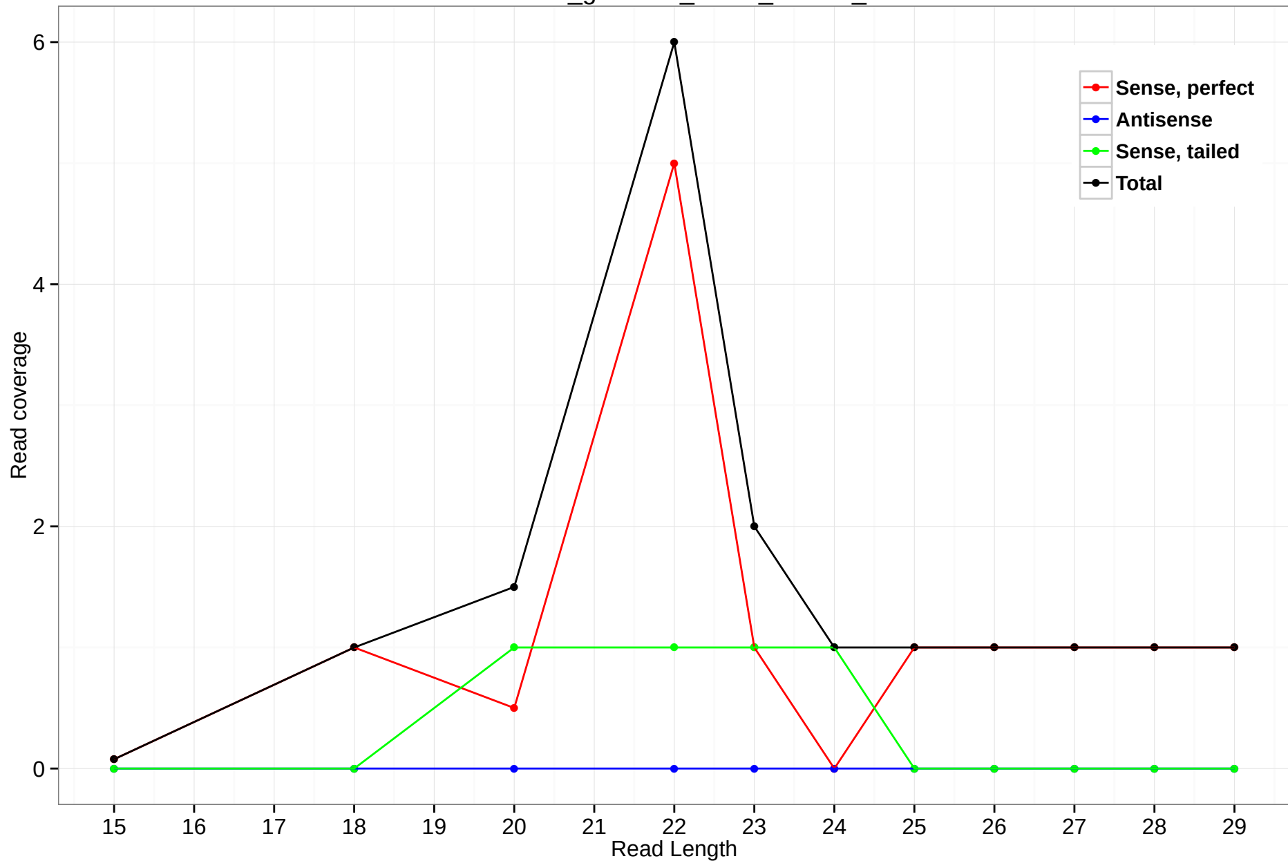
rheMac3_genscan_chr14_05.114_6
