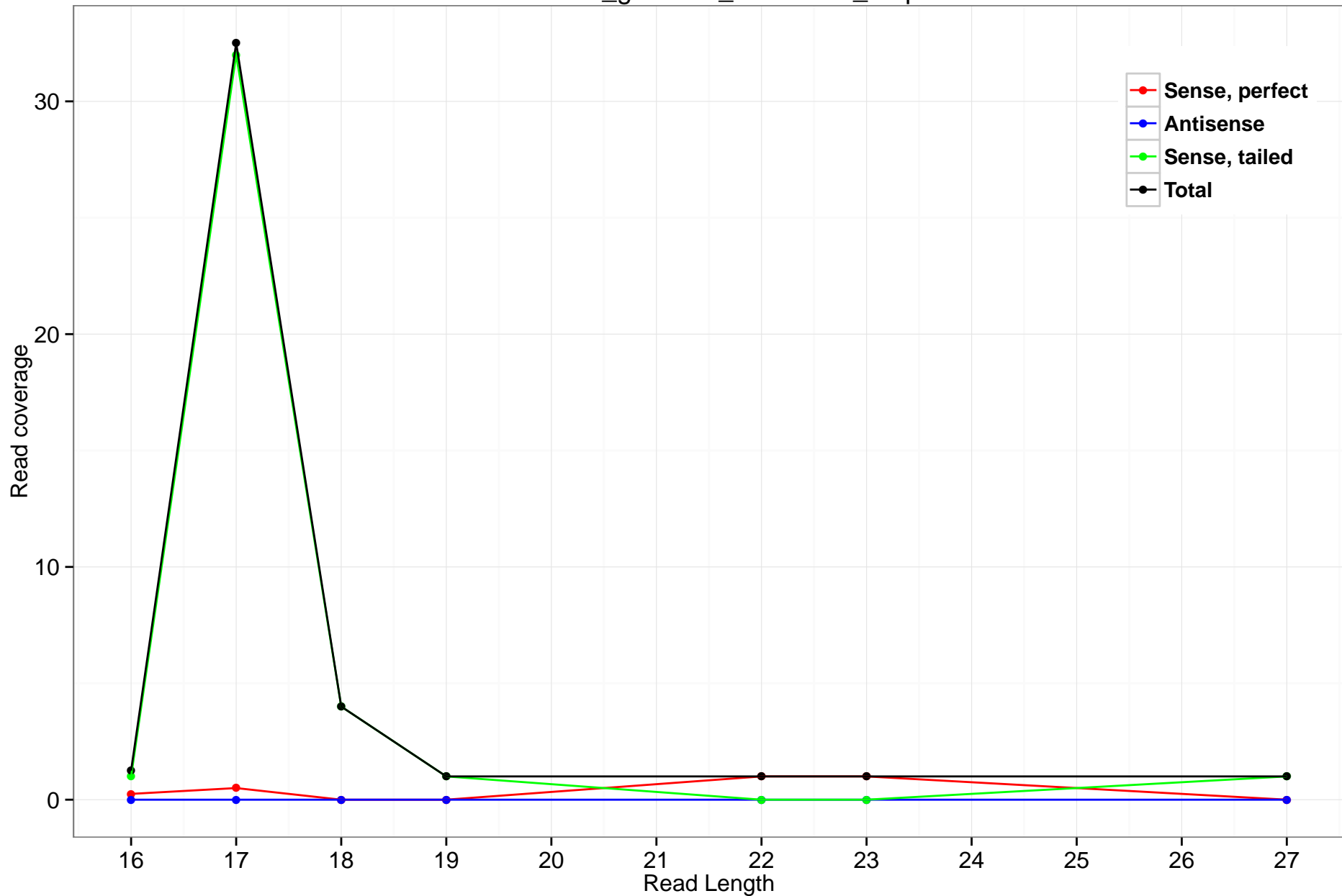
rheMac3_genscan_chr14.335_9.5p
