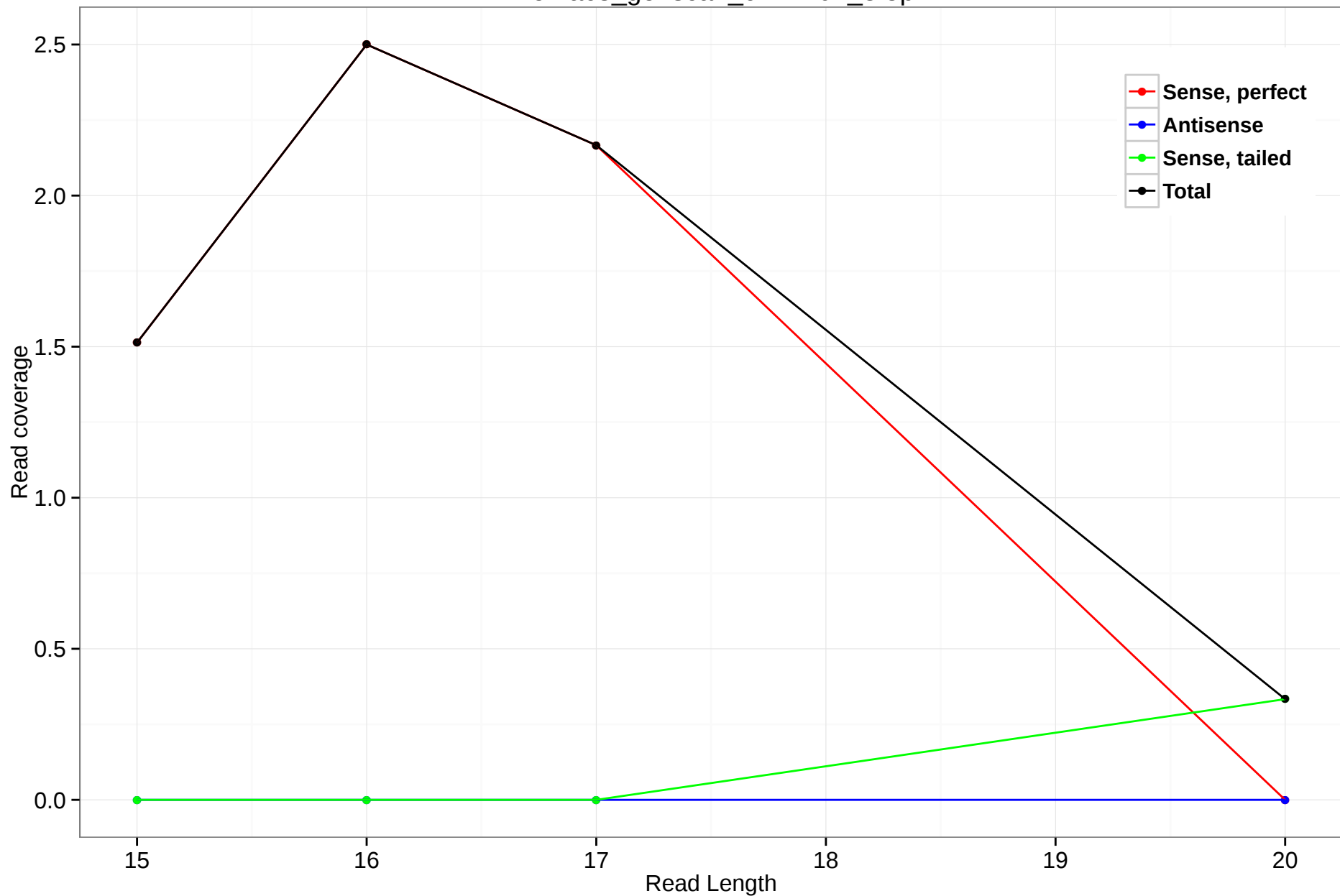
rheMac3_genscan_chr14.07_8.5p
