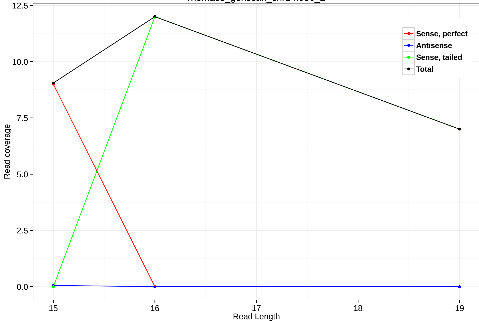
rheMac3_genscan_chr14.036_2
