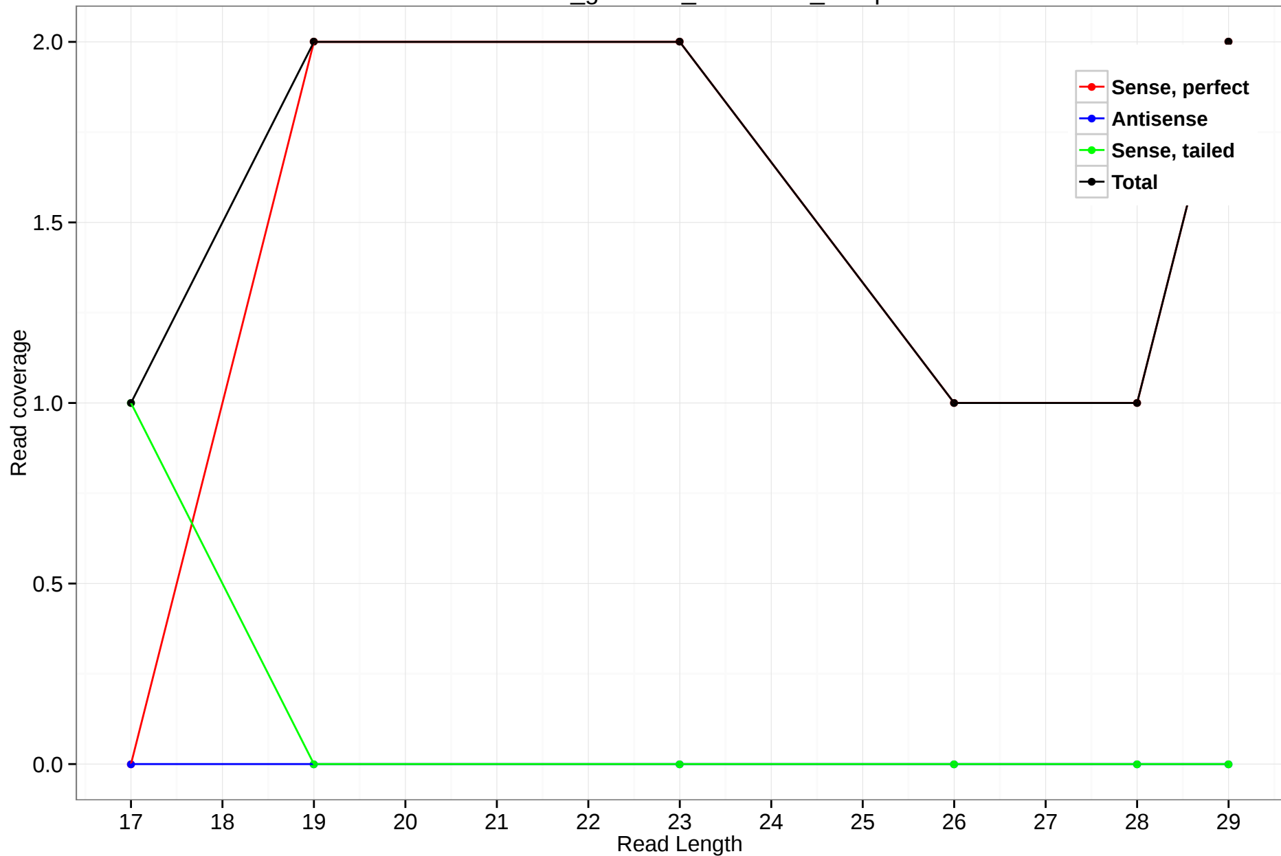
rheMac3_genscan_chr14.033_18.5p
