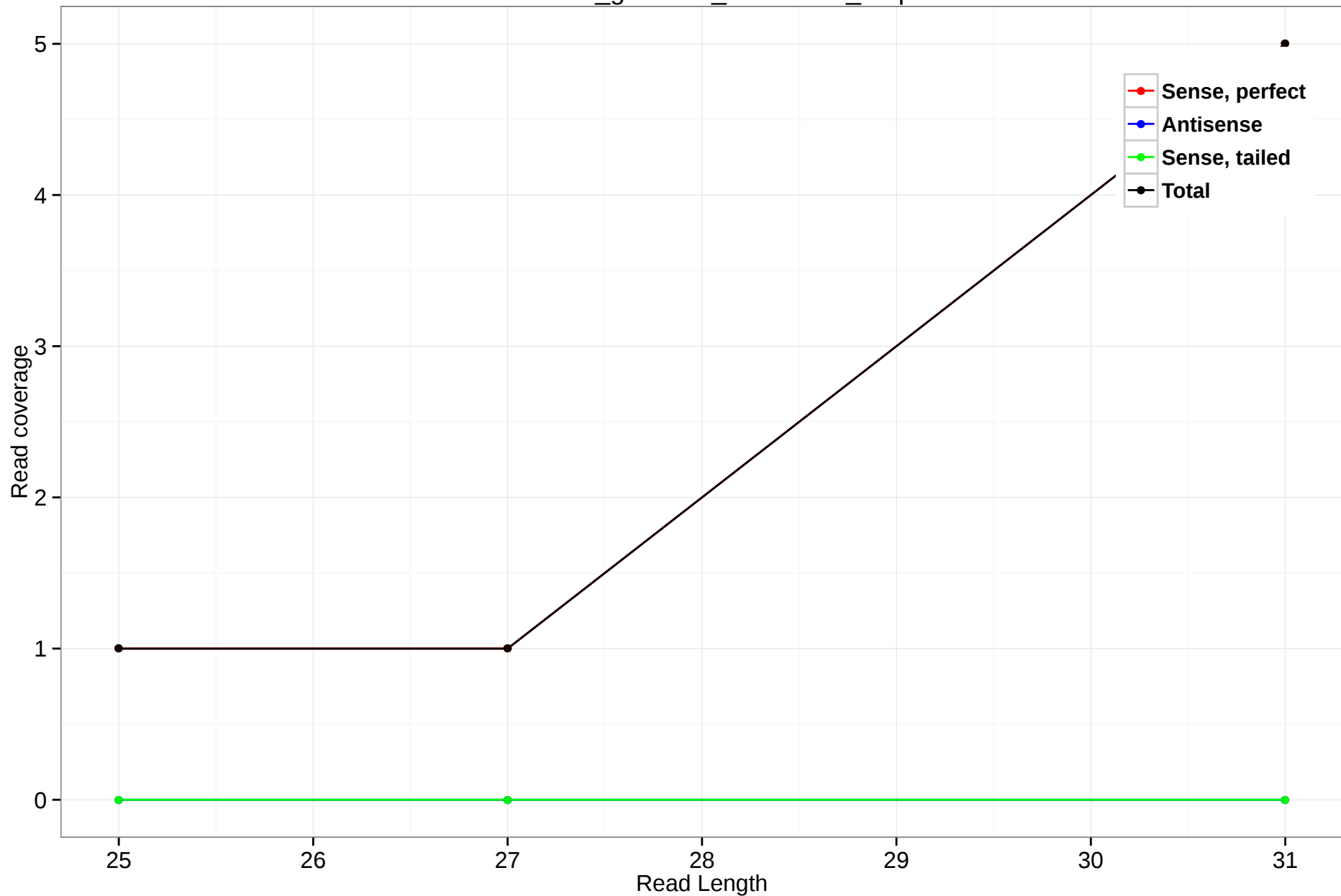
rheMac3_genscan_chr14.030_9.3p
