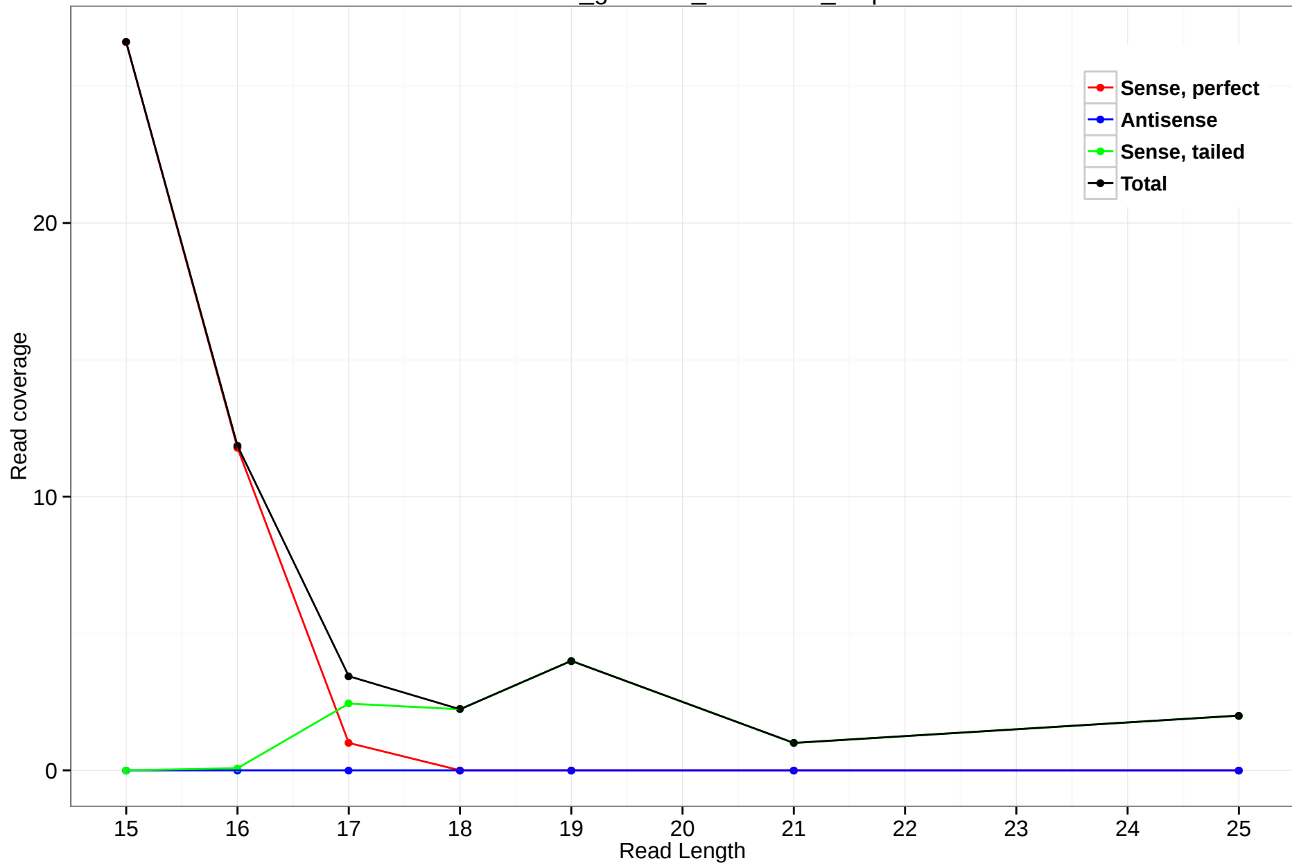
rheMac3_genscan_chr14.029_0.3p
