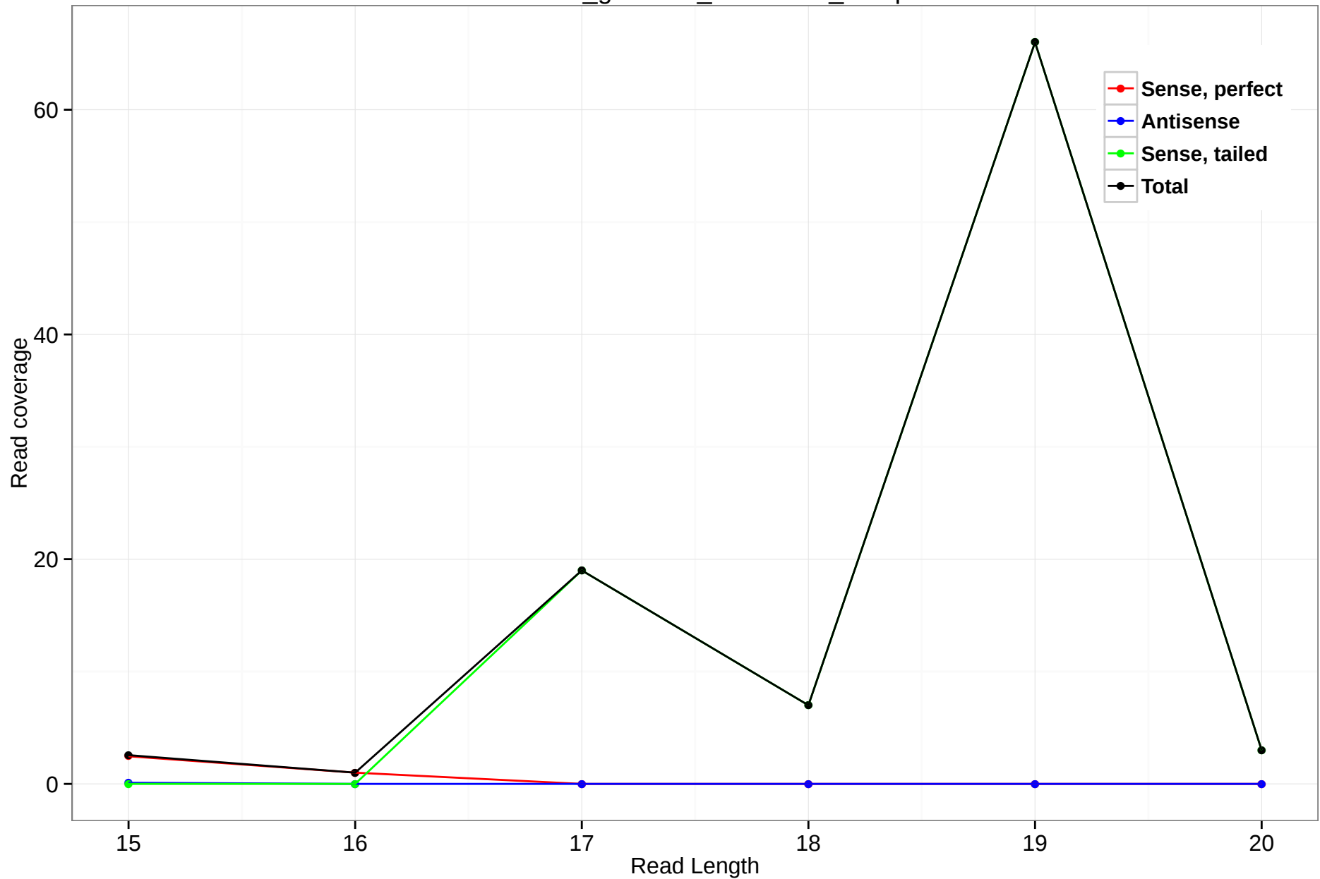
rheMac3_genscan_chr14.019_11.3p
