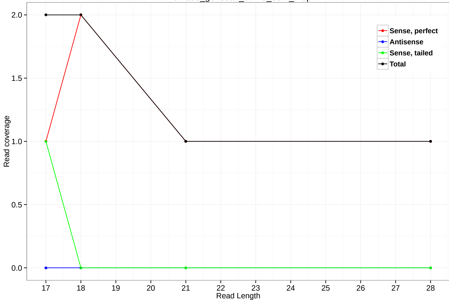
rheMac3_genscan_chr13_85.1_7.3p
