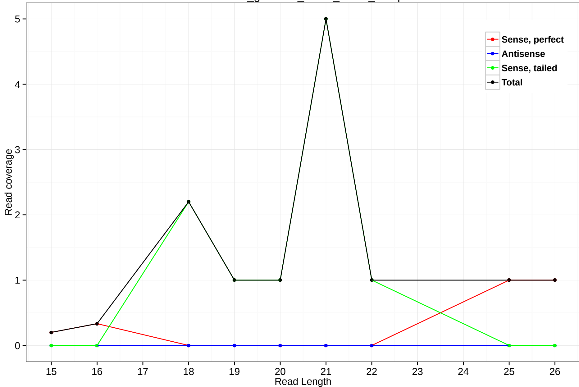
rheMac3_genscan_chr13_85.18_30.3p
