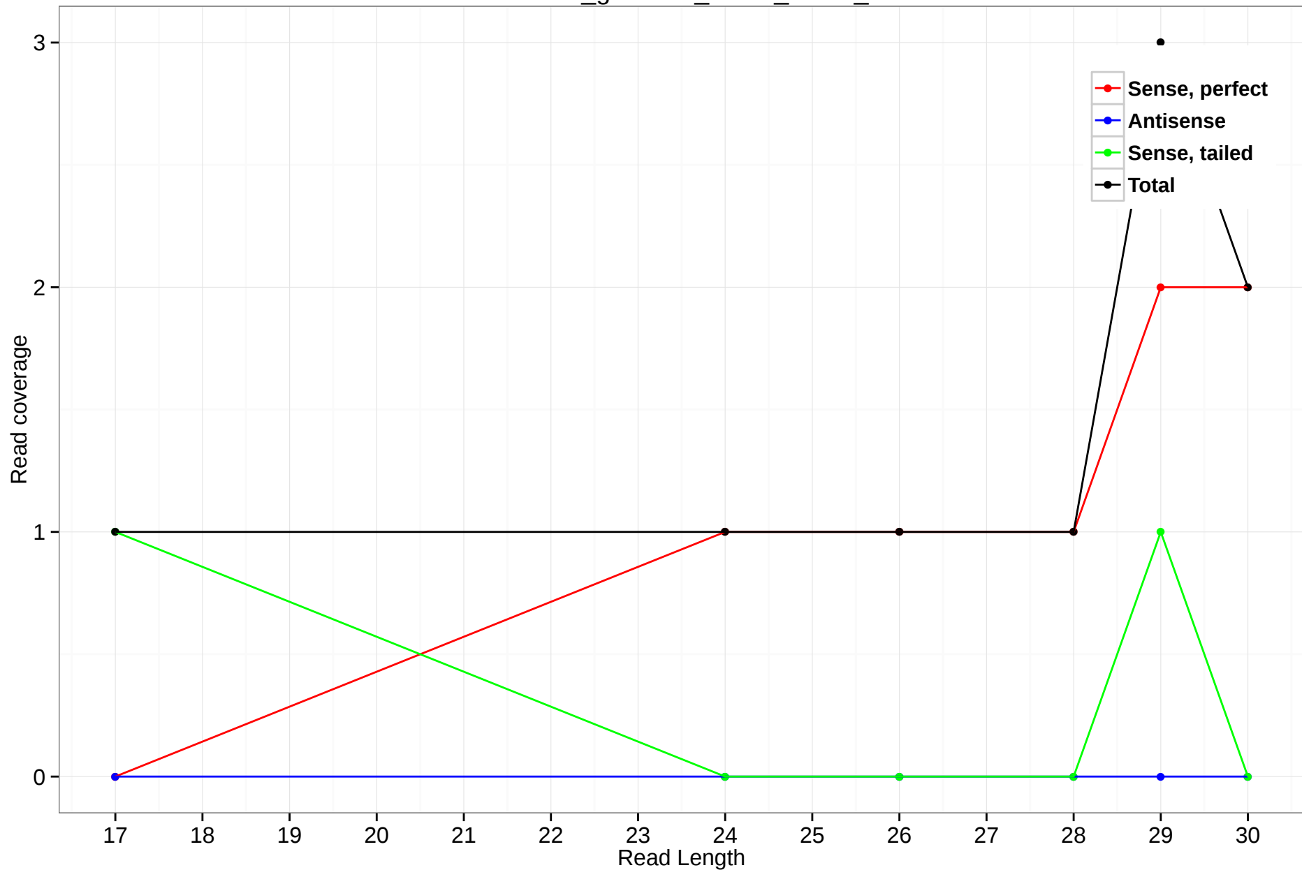
rheMac3_genscan_chr13_58.48_0
